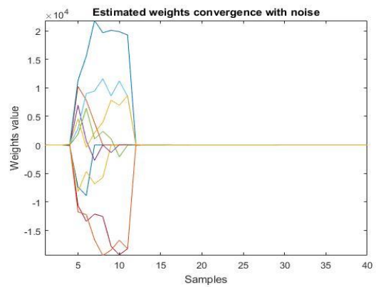
Fig. 16: Estimated weight convergence of IIR Filter with Noise
