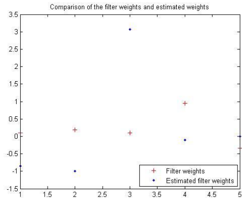
Fig. 10: Comparison of FIR Filter Weights & Estimated weights (Without Noise in ECG Signal)
