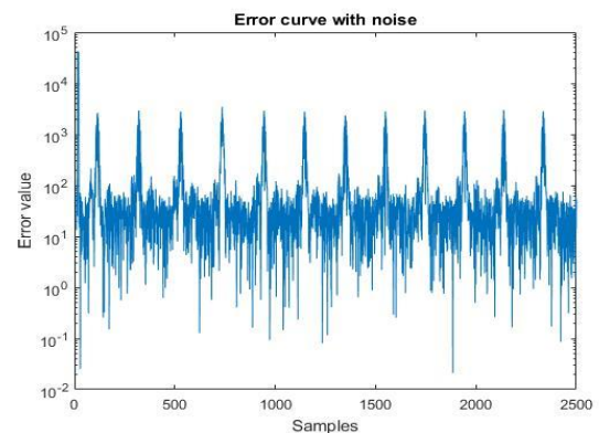
Fig. 9: Error Curve for IIR Filter (With Noise in ECG signal)
