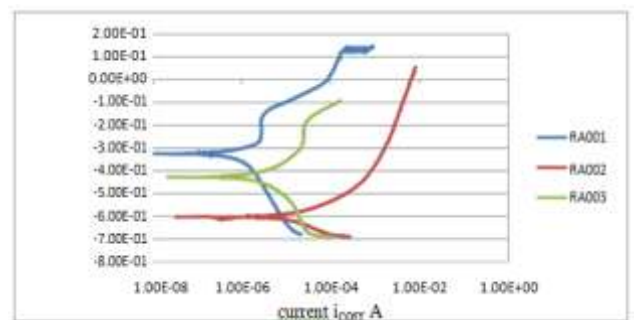
Figure 4.11: Tafel corrosion rate plot of group B in 3.5wt%NaCl solution
