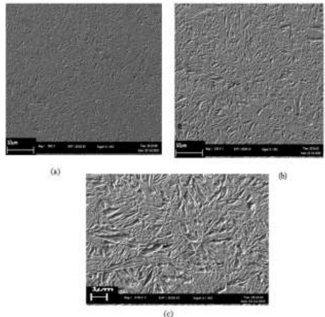
Figure 4.8: Microstructure of low carbon steel after hardening heat treatment (group C) by using SEM (a) 500 x (b) 1000x (c) 2000x magnification
