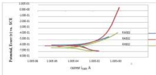
Figure 4.13: Comparison between three group's corrosion rates after 96 hour soaking in 3.5wt%NaCl solution
