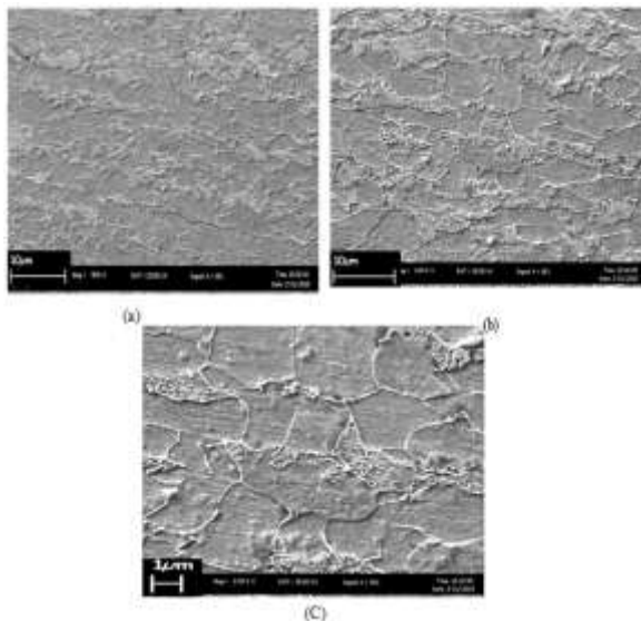
Figure 4.6: Microstructure of low carbon steel without heat treatment (group A) by using SEM (a) 500 x (b) 1000x (c) 2000x magnification
