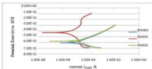
Figure 4.14: Comparison between three group's corrosion rates after 240 hour soaking in 3.5wt%NaCl solution
