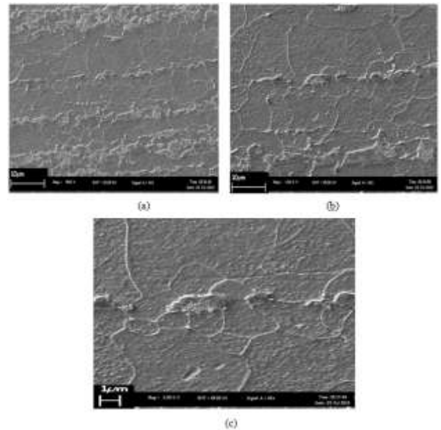
Figure 4.7: Microstructure of low carbon steel after annealing heat treatment (group B) by using SEM (a) 500 x (b) 1000x (c) 2000x magnification
