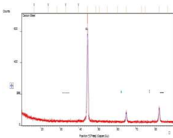
Figure 4.2: X-ray diffraction (XRD) analysis of lowcarbon steel
