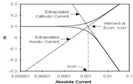
Figure 3.10: Classic Tafel extrapolation (Getting Started with Electrochemical Corrosion Measurement).
