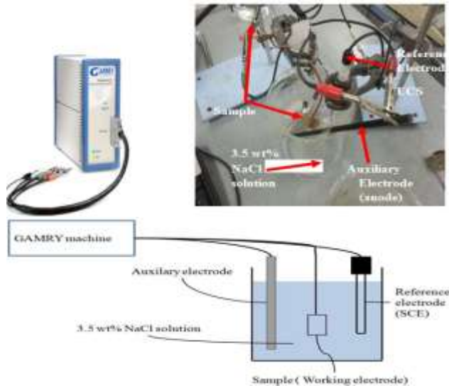
Figure 3.7: Diagram of electrochemical measurement cell
