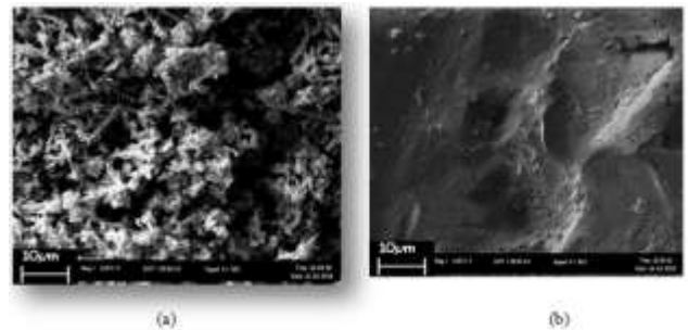
Figure 4.15: The SEM surface morphology of low carbon steel sample without heat treatment after soaking in 3.5 wt% NaCl solution (a) RW002 (b) RW003
