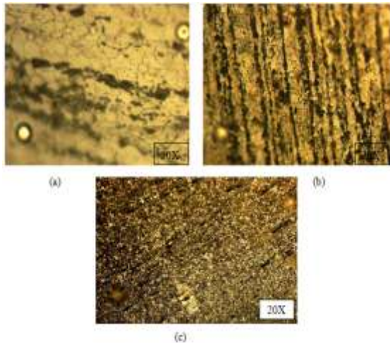
Figure 4.5: Microstructure of low carbon steel without heat treatment by using OM of material (a) As received (b) after annealing (c) after hardening
