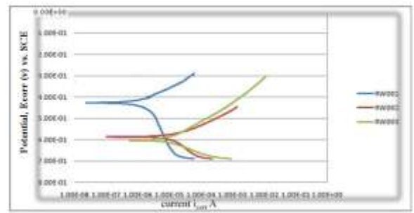
Figure 4.10: Tafel corrosion rate plot of group A in 3.5wt%NaCl solution
