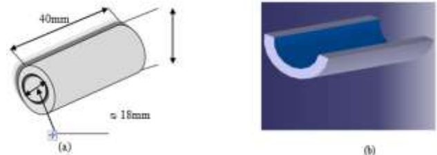
Figure 3.1: Samples shape and dimension (a) before cutting (b) after cutting
