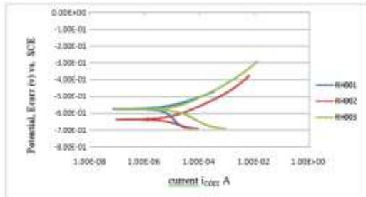
Figure 4.12: Tafel corrosion rate plot of group C in 3.5wt% NaCl solution
