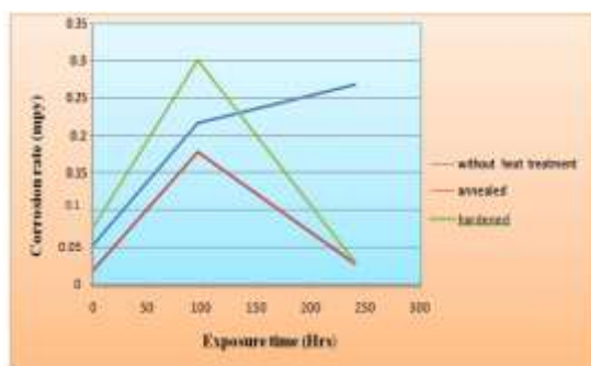
Figure 4.18: Relationship of corrosion behavior between three groups after soaking.
