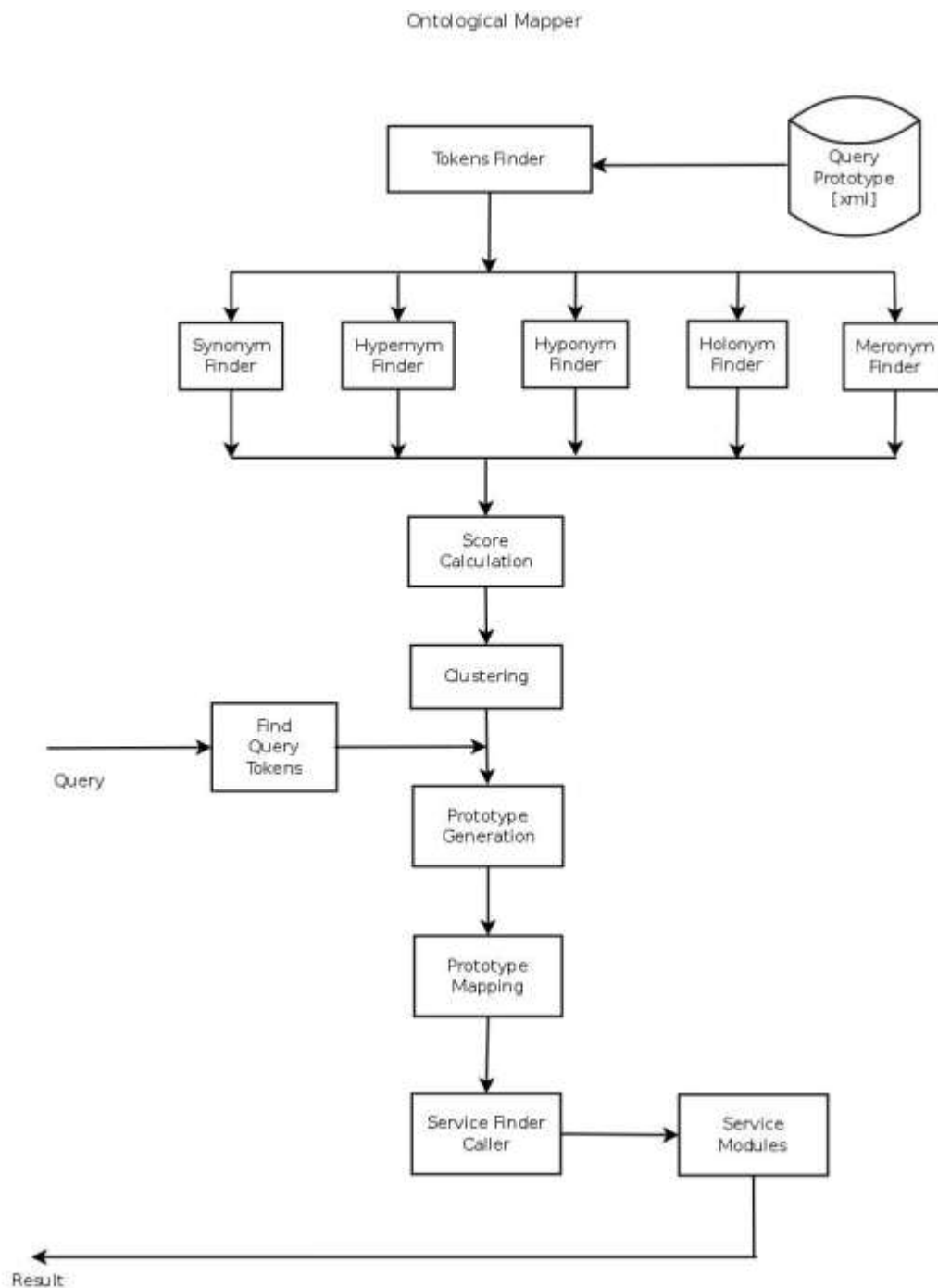
Fig 1: Steps for Ontology Construction
