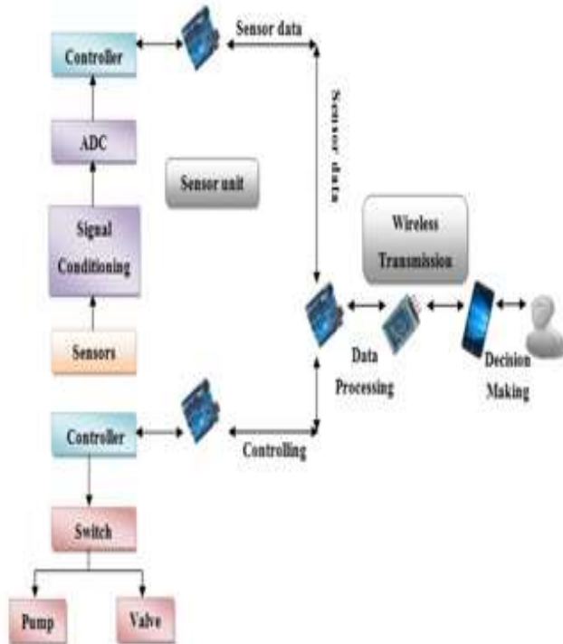
Fig.3: System Architecture
