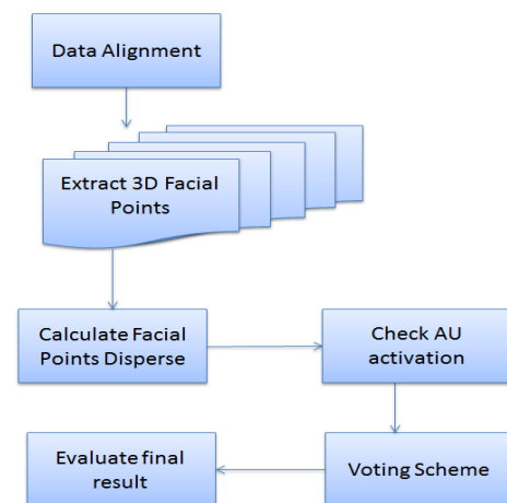
Figure 2 Overview of our work
