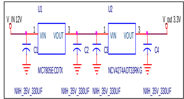
Fig. 5: Interface Circuit Design of Beacon Combined CCTV.
