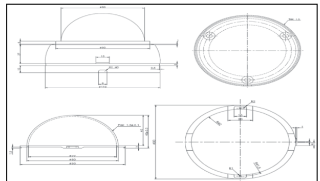
Fig. 7: Actual Survey Drawing of Camera Cover.
