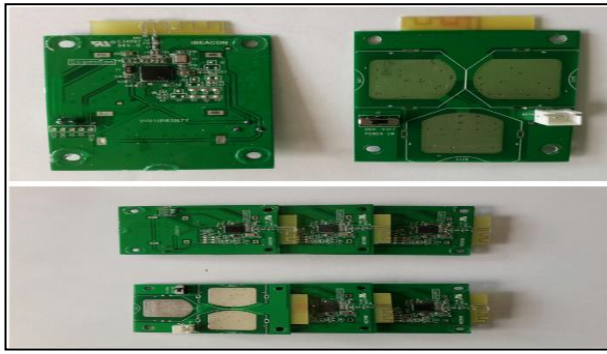
Fig. 3: Picture of PCB in Beacon Signal Transmitter and SMT.
