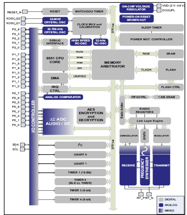
Fig. 1: Block Diagram of CC2541.
