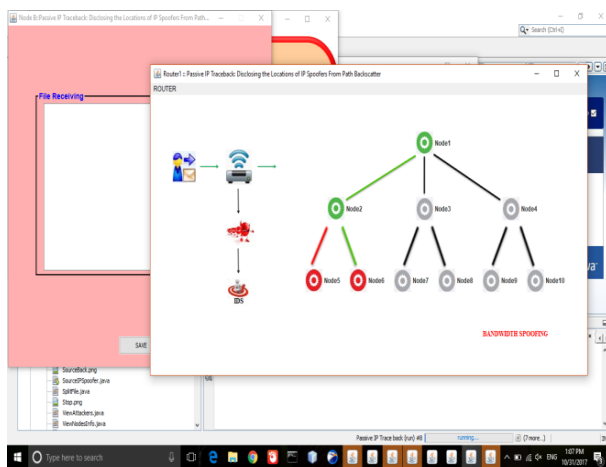
Fig. 11: Here the Node 5 is Rejected and Backtracked to the Previous Node and Checks the Node 6 and where It Is Also Rejected As Shown. and the Reason Why the Node 5 and Node 6 are Rejected is that those Nodes are Not Capable of Sending the Data where There May Be A Defect in the Bandwidth Attained to those Nodes.
