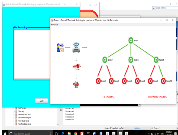
Fig. 22: At This Point the User Is Clearly Under Attack because at Every Node the Data Is Not Received and Says that the Service Is Under Attack, where the IP Address or the Bandwidth are Spoofed by A Fake One.
