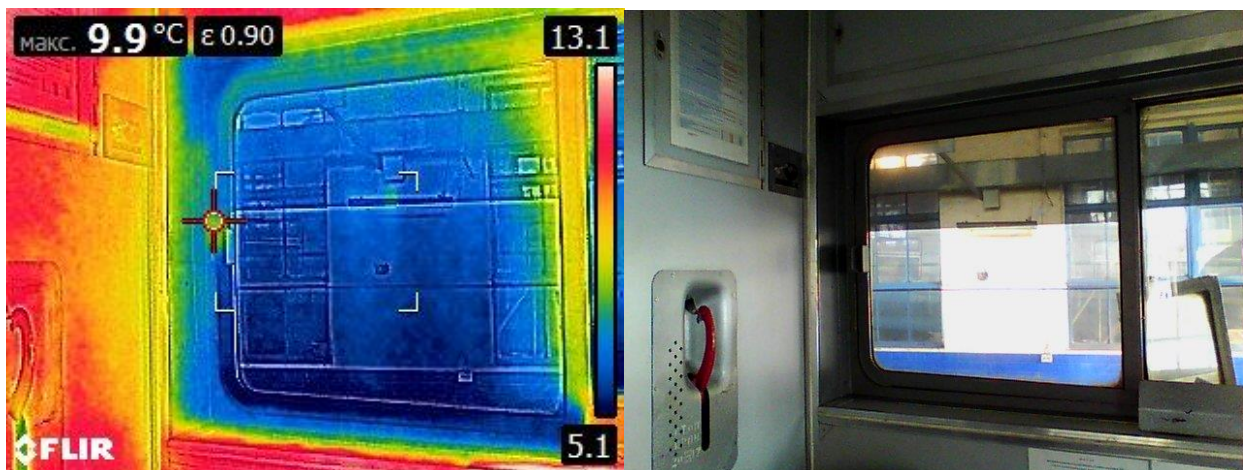
Fig. 4: Thermograms and images of the driver's cabin windows from the driver side (a, b) and from the assistance driver side (c)
