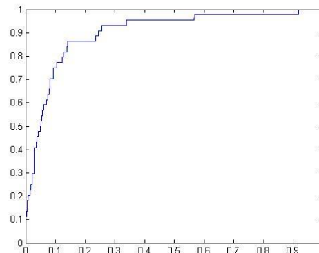
Fig 6: ROC Curve kc2 dataset
