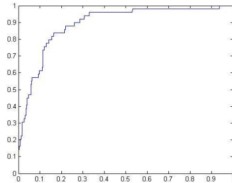
Fig 4: ROC Curve cm1 dataset
