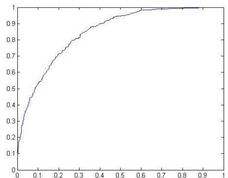
Fig 5: ROC Curve kc1 dataset
