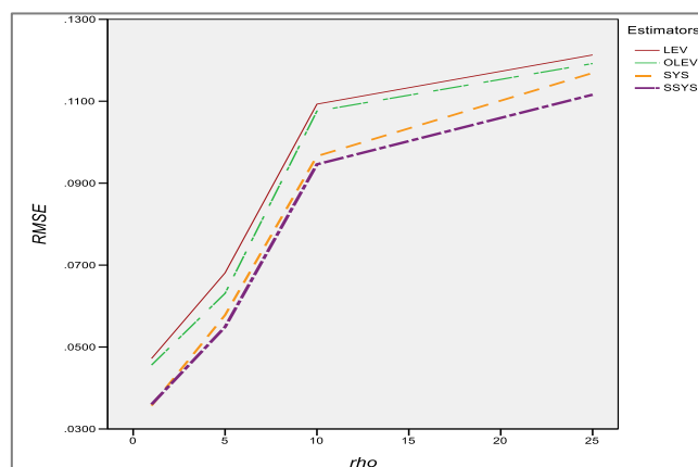
Fig. 2: RMSE of the conventional and new GMM estimators when \phi = .85 , T = 8 , and N = 600 .
