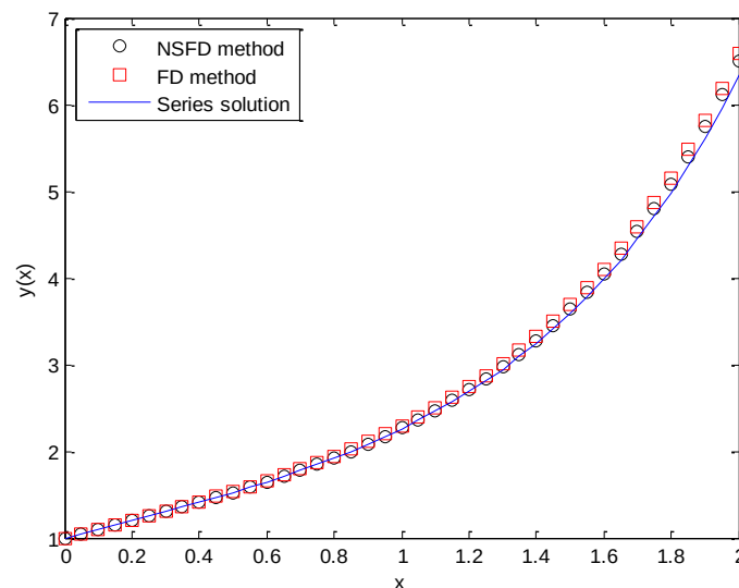
Fig. 7: Numerical Solutions of NSFD and FD Methods for Solving Equation (39) with h = 0.05 .
