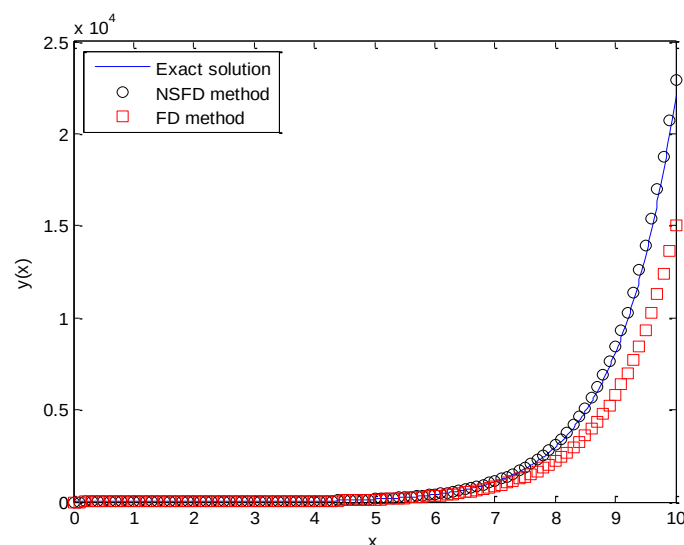
Fig. 2: Numerical Solutions of NSFD and FD Methods for Solving Equation (13) with h = 0.1 .
