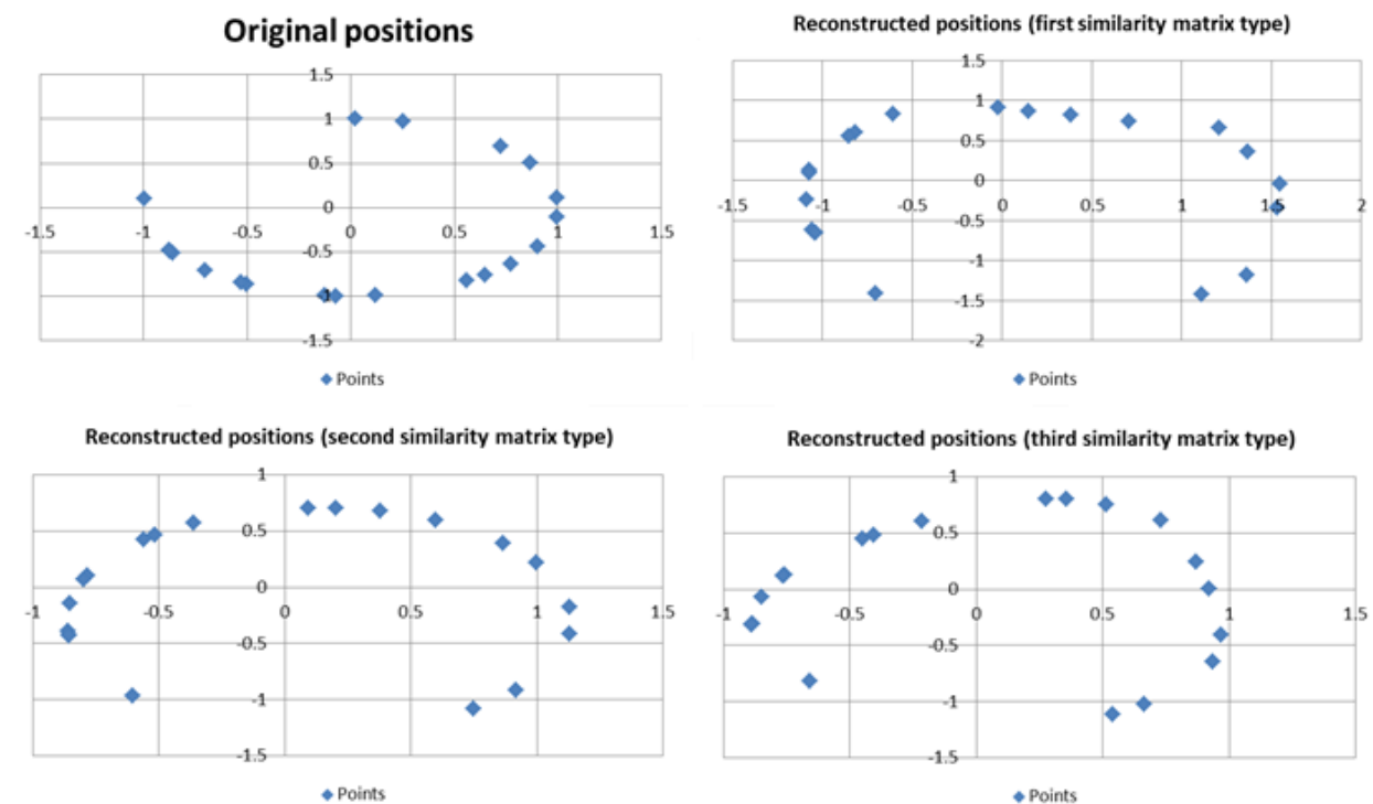
Fig. 7: The original and reconstructed structures of the 20-point test problem using (l_2, l_2) reconstruction models.
