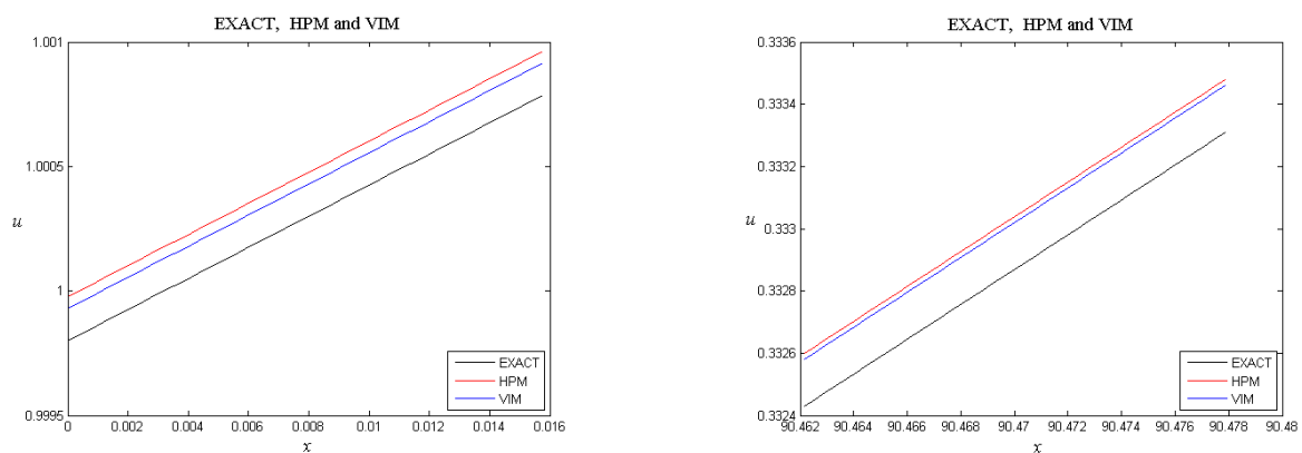
Fig. 4: The zoom curve shows the solution u(x, t) of exact solution, 3 rd Order of (HPM) and 3 rd Order of (VIM): (A) when x \in [0, 0.005\pi] , t = 0.0004 , (B) when x \in [28.795\pi, 28.8\pi] , t = 0.0004 .
