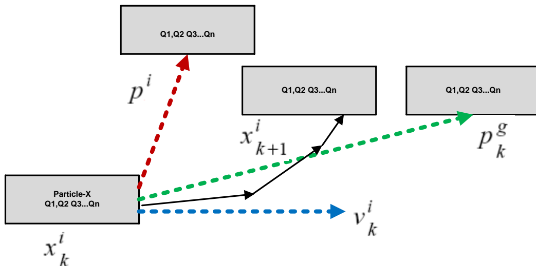
Figure 2 PSO mechanism over N-Queens problem
