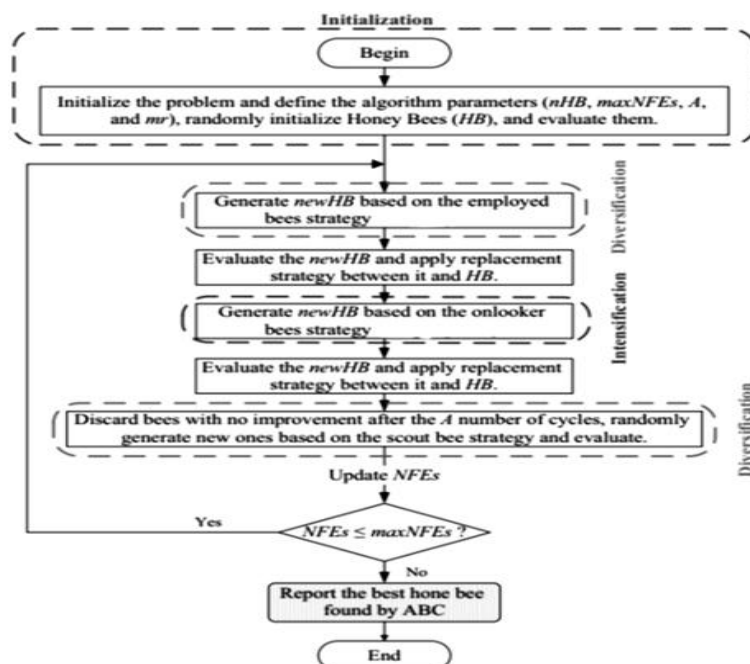
Fig. 2: ABC Algorithm Flowchart.
