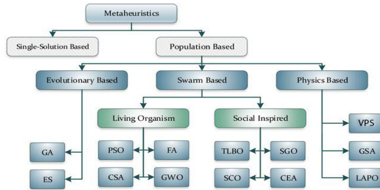
Fig. 1: Metaheuristics Algorithms Classifications [1].
