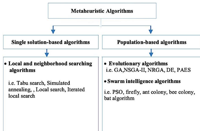
Fig. 1: Metaheuristic Classifications.
