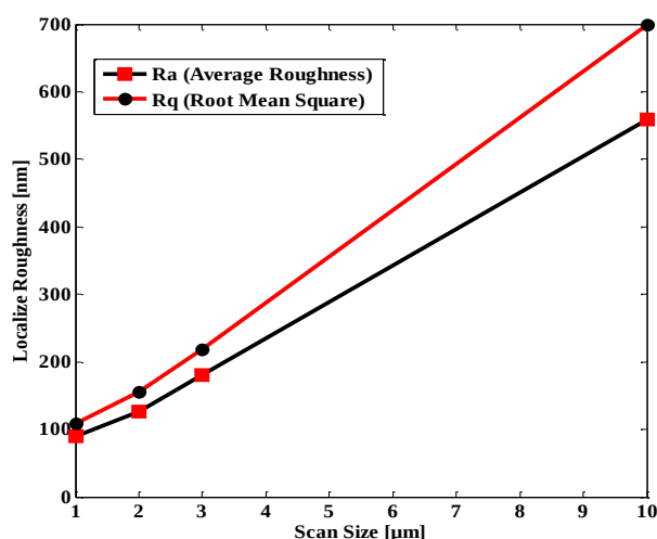
Fig. 9: Roughness Data for the Textured Sample at Different Etch Temperature.
