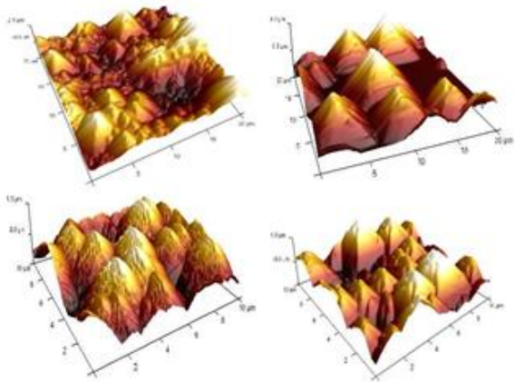
Fig. 4: 3 D Profile AFM Images of KOH Textured Silicon Wafer Samples at Different Etchant Concentration.
