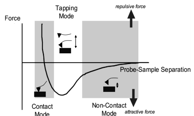
Fig. 2: Plot of Force as a Function of Probe-Sample Separation.
