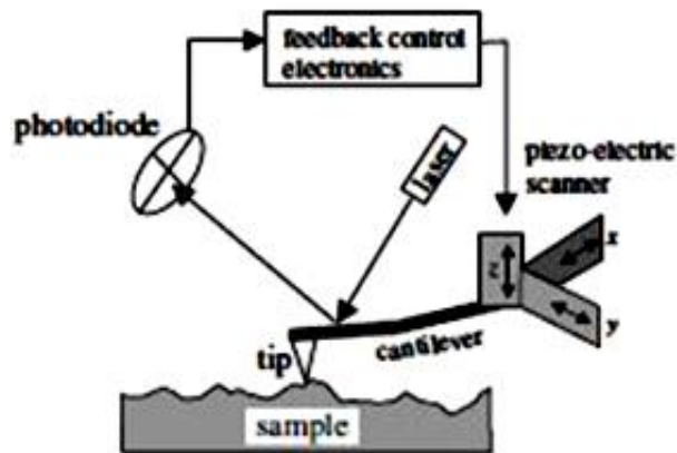
Fig. 1: Schematic Diagram of an Atomic Force Microscope.
