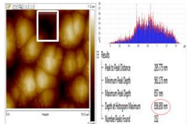
Fig. 7: Presents A Top View Image, A Histogram and Depth Data Results from Raw Depth Data for an Optimally Textured Silicon Substrate.
