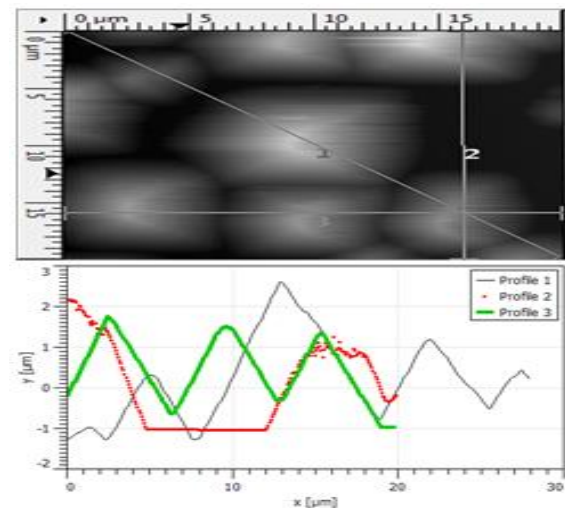
Fig. 6: 2 D Atomic Force Microscopic (AFM) Height and Cross-Sectional Images for A KOH Textured Wafer Sample Using the Gwyddion Software Package.
