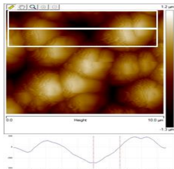
Fig. 10: Step Height Analysis of AFM Image of A Textured Silicon Wafer (A Step Height of 19.0 Nm Was Obtained) as Shown Above, By Analyzing Cross Sectional Plots the Difference between the Average Height of Each Region.
