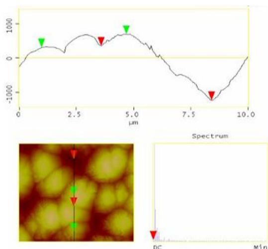
Fig. 5: 2 D Atomic Force Microscopic (AFM) Height and Cross-Sectional Images for A KOH Textured Wafer Sample under the Condition: KOH=40%, T=80°C, T=40 Min.
