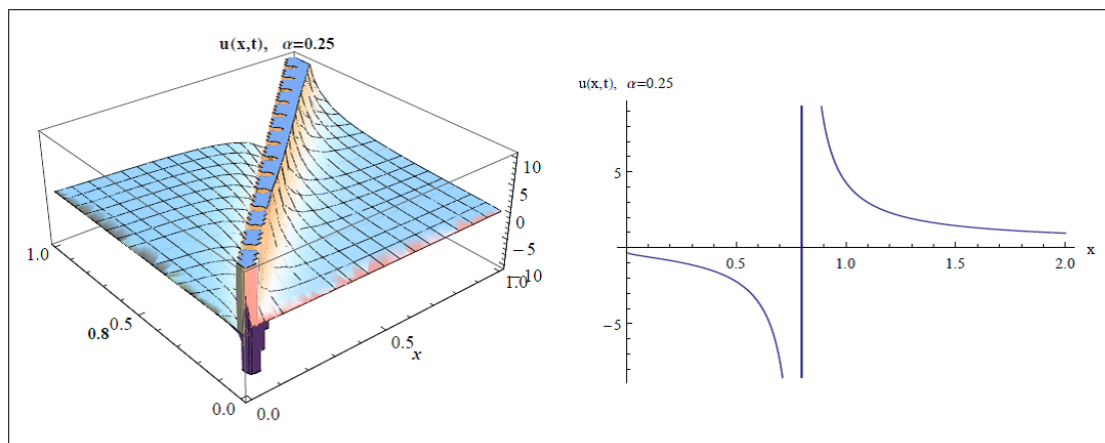
Fig. 6: Profiles of Eq. (21), Substituting the Values of the Parameters a_1 = 2.8, p = 3, q = 1, r = 0, \alpha = 0.25 and t = 0.25 for 2D Graph.
