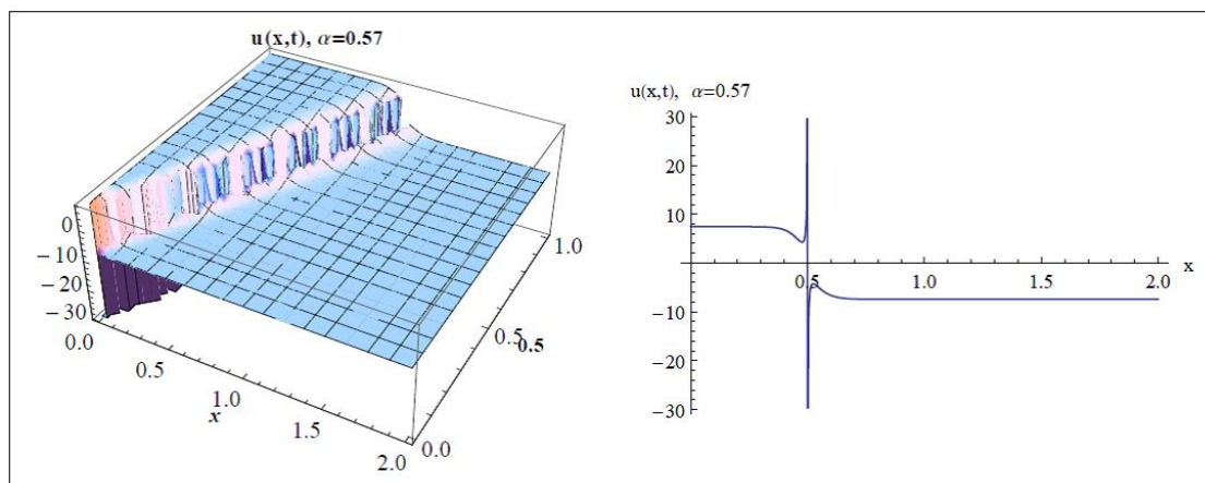
Fig. 7: Profiles of Eq. (22), Substituting the Values of the Parameters a_1 = 1.8, b_1 = 1.2, p = 2, q = 1, a = 1.2, \alpha = 0.57 and t = 2.4 for the 2D Graph.
