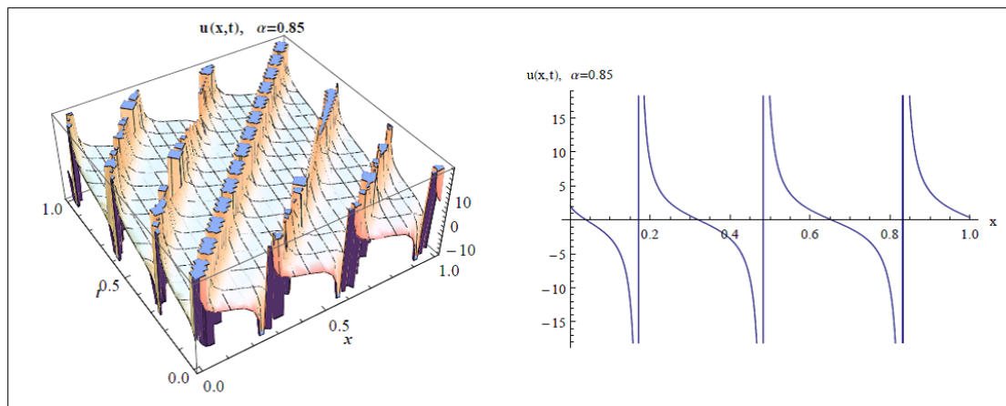
Fig. 5: Profiles of Eq. (20), Substituting the Values of the Parameters a_1 = 2.3, p = 2, q = 1, r = 1.5, \alpha = 0.85 and t = 2 for the 2D Graph.
