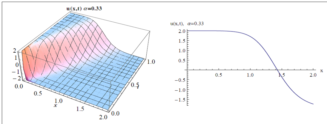
Fig. 1: Profiles of Eq. (13), Substituting the Values of the Parameters p = 2; q = 0.2, a_0 = 2; d = 0.7; \alpha = 0.33 , and t = 1 for the 2D Graphs.
