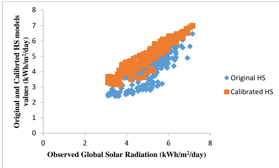
Fig. 3: Comparison of Monthly Observed H Values, Original HS and Calibrated HS Models in Each Station of Nigeria
