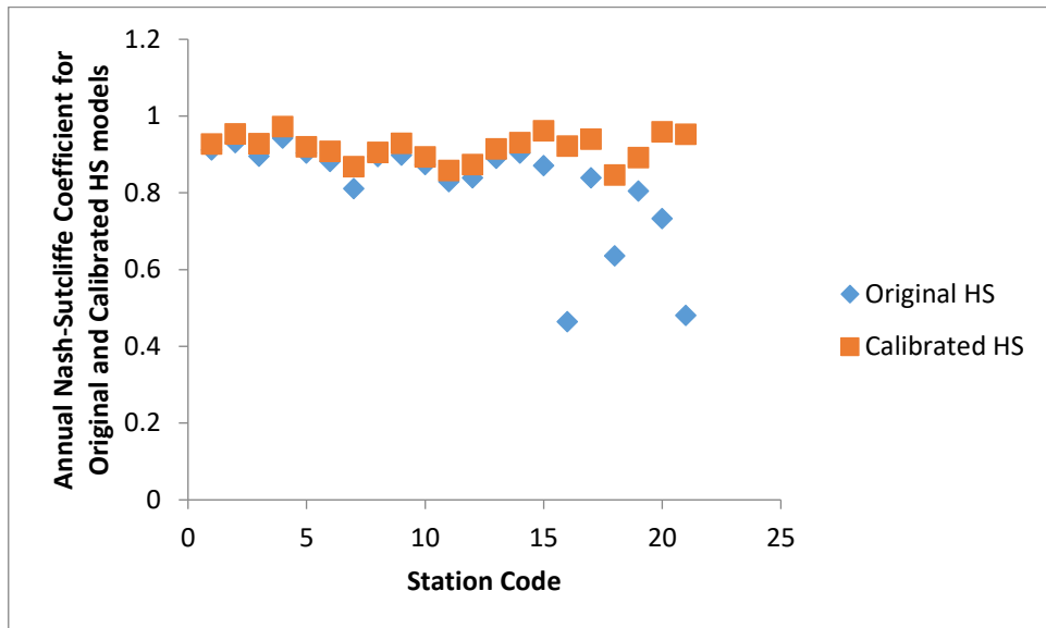
Fig. 7: Comparison of Annual Nash-Sutcliffe Coefficient (NS) of Original and Calibrated HS Models with Station Code for All Stations.
