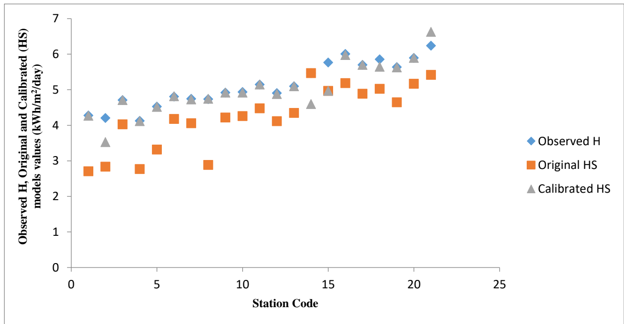
Fig. 2: Comparison of Annual Observed H Values, Original HS and Calibrated HS Models in Each Station of Nigeria.
