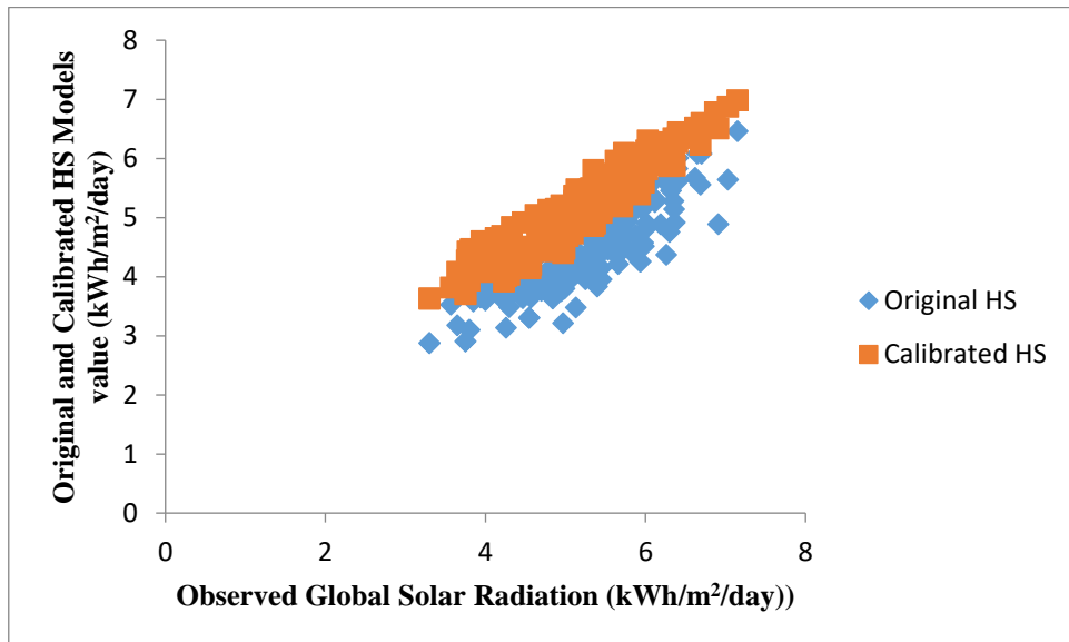
Fig. 4: Comparison of Monthly Observed H Values, Original HS and Calibrated HS Models for Interior Region of Nigeria.
