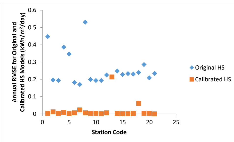
Fig. 9: Comparison of Annual RMSE of Original and Calibrated HS Models with Station Code for All Stations.
