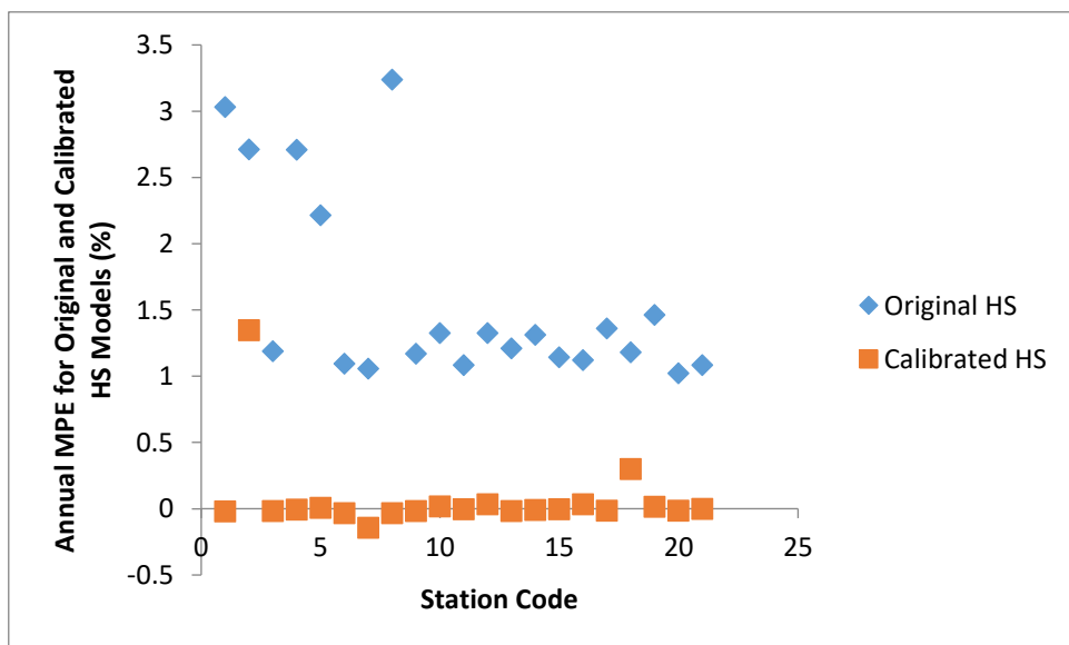
Fig. 8: Comparison of Annual MPE of Original and Calibrated HS Models with Station Code for All Stations.
