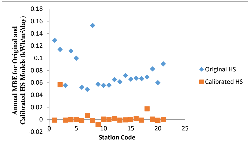
Fig. 6: Comparison of Annual MBE of Original and Calibrated HS Models with Station Code for All Stations.
