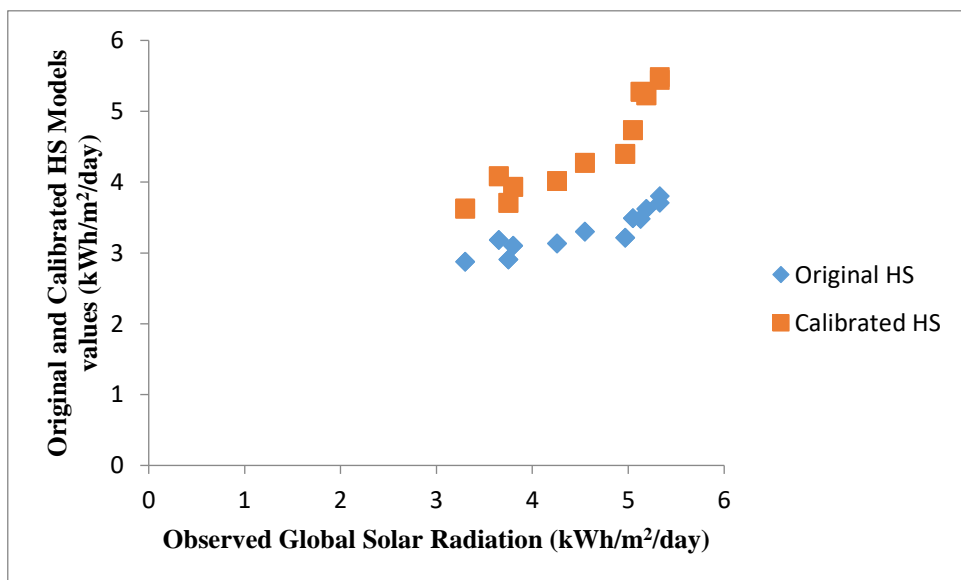
Fig. 5: Comparison of Monthly Observed H Values, Original HS and Calibrated HS Models for Coastal Region of Nigeria.
