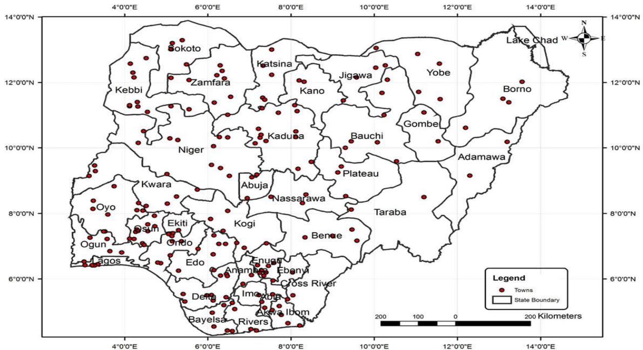
Fig. 1: Map of Nigeria Showing the Geographical Stations of the Cities Used in this Study.
