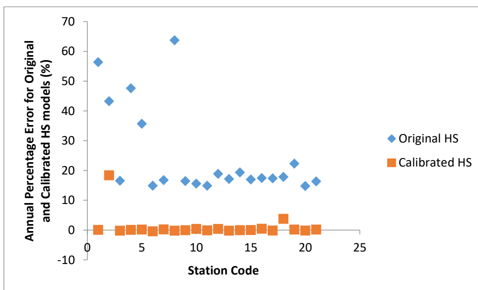
Fig. 10: Comparison of Annual Percentage Error of Original and Calibrated HS Models with Station Code for All Stations.
