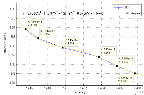
Fig. 6: The Variation of Refractive Indices Depending on HbO 2 Resonance Peaks.
