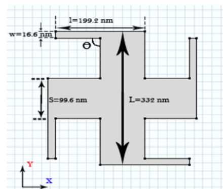
Fig. 2: Chiral Metamaterials Structure.
