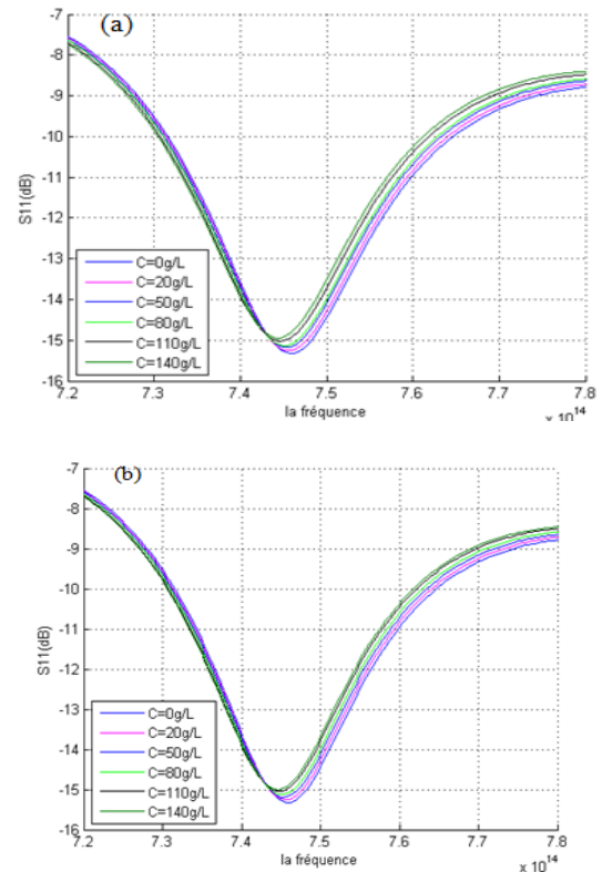
Fig. 5: (A) - The Variation of the Resonance Peaks Depending on the Refractive Indices of HbO 2 , (B) - Variation of the Resonance Peaks Based on Hb Refractive Indices.
