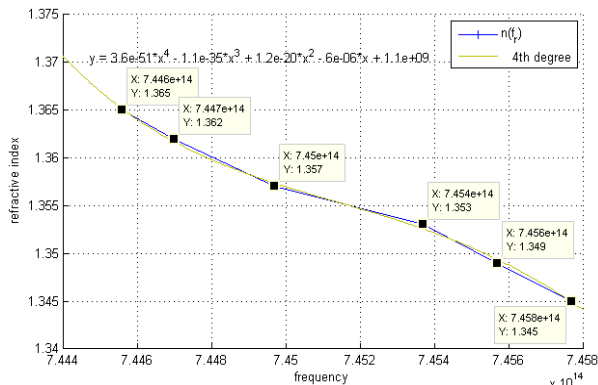
Fig. 8: The Variation of Refractive Indices Depending on Hb Resonance Peaks.
