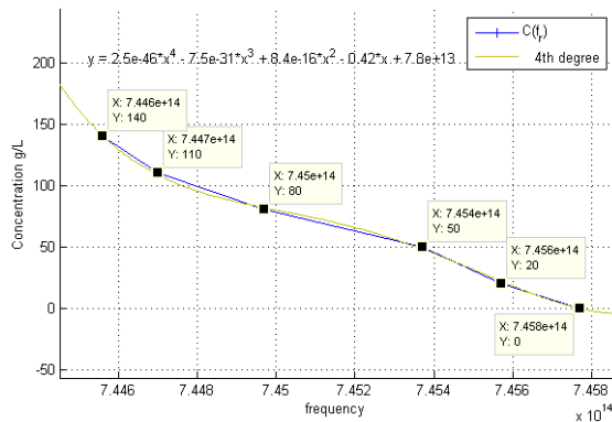
Fig. 7: The Variation of the Concentration Depending on HbO 2 Resonance Peaks.
