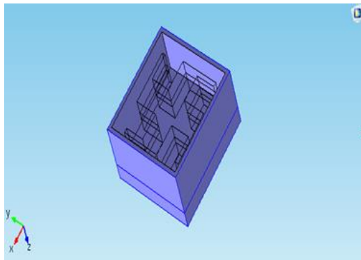
Fig. 3: Representation of the Structure MMC Nano-Sensor without the Hemoglobin.
