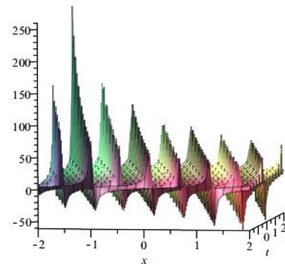
Fig. 5: 3D Graphics (Periodic Profile) of Solutions Eq. (28) when \alpha_0=5, k=-0.8, r=-1, \beta=2, \lambda=2, \mu=3, m=1, y, A=0 and -2 \leq x, t \leq 2
