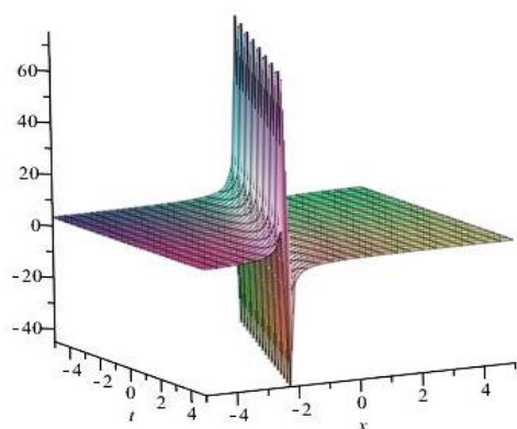
Fig. 8: 3D Graphics (Singular Kink Profile) of Solutions Eq. (34) when \alpha_0 = 3, k = 1.5, r = -0.5, \beta = 1, \lambda = 2, \mu = 1, m = 1, y = 0, A = 1, B = 1 And -5 \leq x, t \leq 5 .
