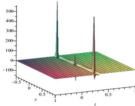
Fig. 1: 3D Graphics (Soliton Profile) of Solutions Eq. (21) when \alpha_0=3, k=0.8, r=2, \beta=5, \lambda=3, \mu=1, m=1, y=0, A=5 and -0.5 \leq x, t \leq 1
