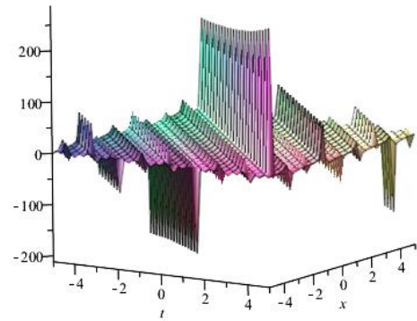
Fig. 4: 3D Graphics (Periodic Profile) of Solutions Eq. (49) when \alpha_0=3, k=1, r=1, \beta=3, \lambda=1, \mu=2, m=0.5, y=0, A=5 and -5 \leq x, t \leq 5 .
