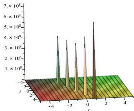
Fig. 7: 3D Graphics (Soliton Profile) of Solutions Eq. (55) when \alpha_0=3, k=1.5, r=-0.5, \beta=3, \lambda=2, \mu=1, m=1, y=0, A=5, B=1 and -5 \leq x, t \leq 5 .
