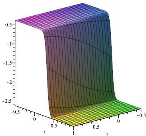
Fig. 2: 3D Graphics (Kink Profile) of Solutions Eq. (24) when \alpha_0=3, k=0.8, r=2, \beta=5, \lambda=3, \mu=1, m=1, y=0, A=5 and -0.5 \leq x, t \leq 1 .
