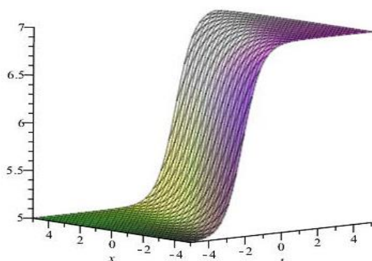
Fig. 9: 3D Graphics (Singular Kink Profile) of Solutions Eq. (56) when \alpha_0 = 3, k = 1.5, r = -0.5, \beta = 3, \lambda = 2, \mu = 1, m = 1, y = 0, A = 5, B = 1 And -5 \leq x, t \leq 5 .
