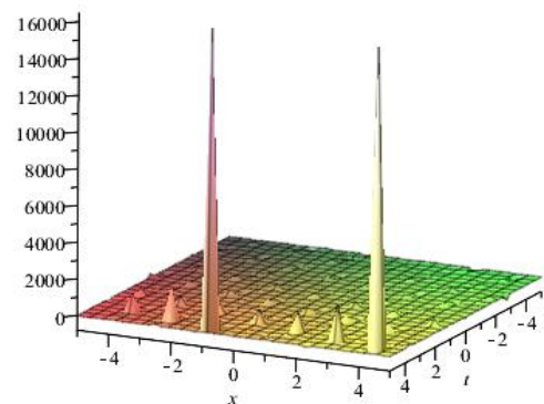
Fig. 6: 3D Graphics (Soliton Profile) of Solutions Eq. (53) when \alpha_0=3, k=1, r=1, \beta=3, \lambda=1, \mu=2, m=0.5, y=0, A=5 and -5 \leq x, t \leq 5 .
