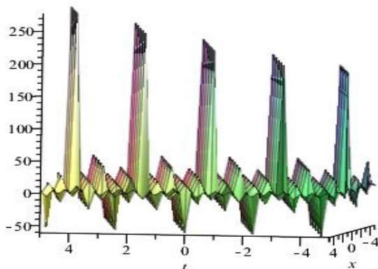
Fig. 3: 3D Graphics (Periodic Profile) of Solutions Eq. (27) when \alpha_0=3, k=1, r=1, \beta=2, \lambda=1, \mu=2, m=0.5, y=0, A=5 and -5 \leq x, t \leq 5 .
