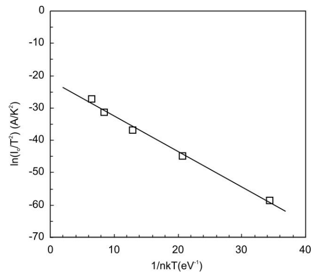
Fig. 2: \ln(I_0/T^2) Dependence on 1/Nk_B T for Ni/4H-SiC Schottky Diode.
