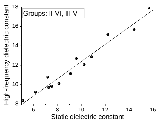
Fig. 2: Scatterplot Of \epsilon_{\infty} and \epsilon_0 Data, plus Fitted Straight Line in II-VI and III-V Zincblende Compounds.
