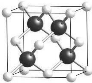
Fig. 1: Position Occupied by Each Atom in Cubic Zincblende Structure. The Structure Consists of the Interpenetrating FCC Lattices, One Displaced from the other by A Distance (1/4, 1/4, 1/4) Along the Body Diagonal [15].
