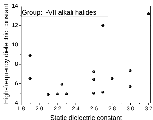
Fig. 3: Scatterplot Of \epsilon_{\infty} and \epsilon_0 Data in I-VII Alkali Halides Compounds.
