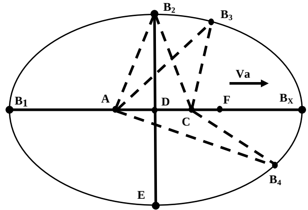
Fig. 7: The Elliptical Law of A Mirrored Signal in A Moving Medium.
