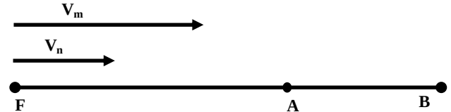
Fig. 3: Matching Speed Case.
