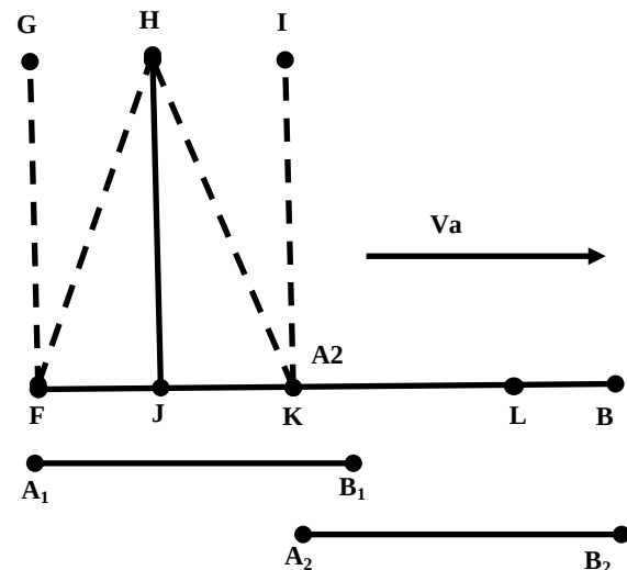
Fig. 5: The Problem of Orthogonal Motion
