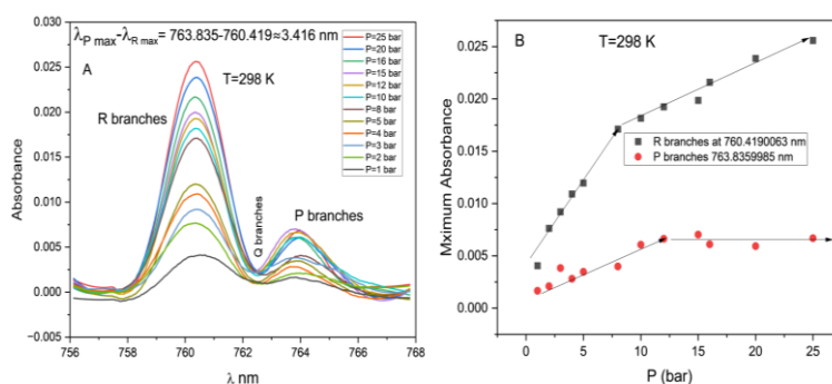
Fig. 10: A) Savitzky-Golay Method to Separate P and R Branches, Fig. 10 B) Absorbance of P and R Branches as A Function of Pressures.
