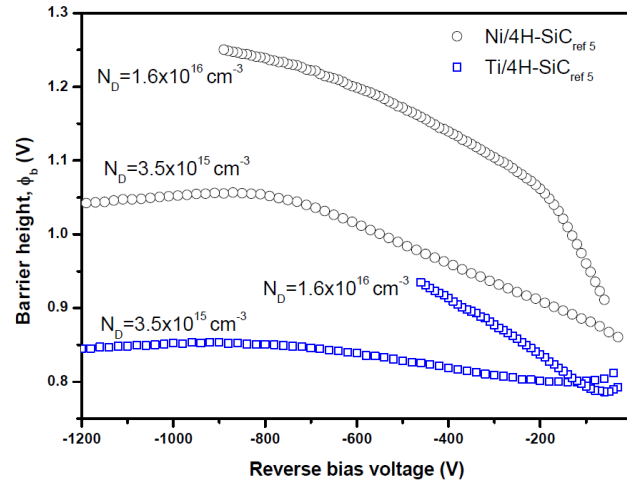
Fig. 7: The Effect of the Metal Nature on the Schottky Barrier Height.
