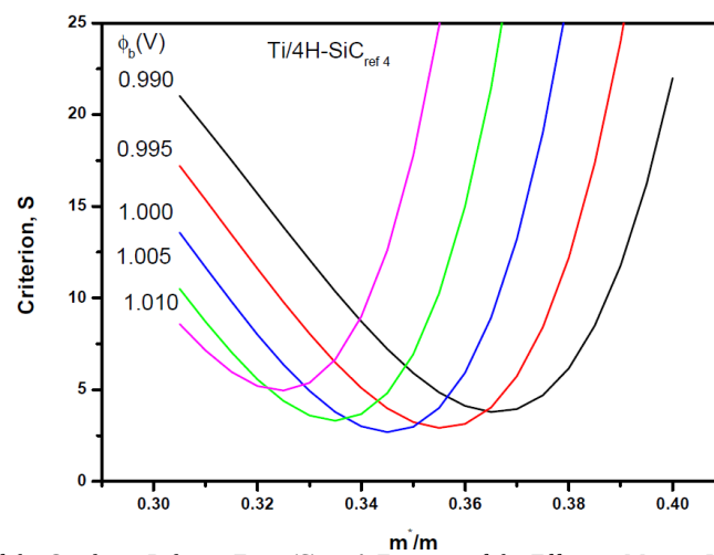
Fig. 3: Minimizing of the Sum of the Quadratic Relative Error (S) as A Function of the Effective Mass at Various Schottky Barrier Heights for the Reverse I -V Data of the Ti/4H-SiC ref 4 SD.
