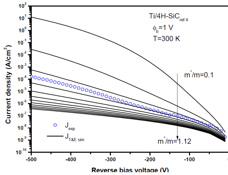
Fig. 2: Current Density Calculated with Tsu-Esaki's Expression as A Function of the Reverse Bias Voltage at Various Effective Mass. with \phi_b = 1 V, T = 300 K.
