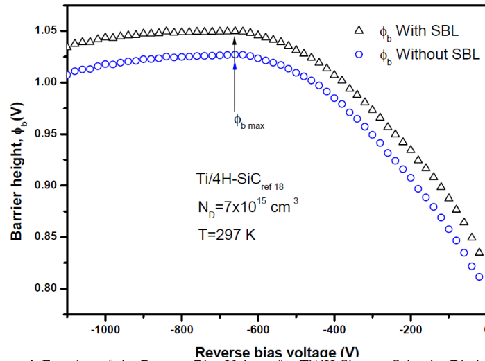
Fig. 5: Schottky Barrier Height as A Function of the Reverse Bias Voltage for Ti/4H-SiC ref 18 Schottky Diode with and Without Schottky Barrier Lowering Effect. The Values of \phi_b Are Extracted By the Tsu-Esaki Model.
