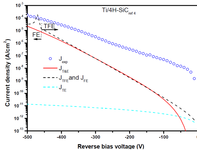
Fig. 1: Comparison of Calculating Current Densities (Thermionic Emission, Field Emission, Thermionic Field Emission and Tsu-Esaki's Expression Calculated With \phi_b^{I-V} = 1.21 \text{ V} ) and Experimental Leakage Current For Ti/4H-SiC ref 4 Schottky Diode. the Experimental Results are From Furno [4].
