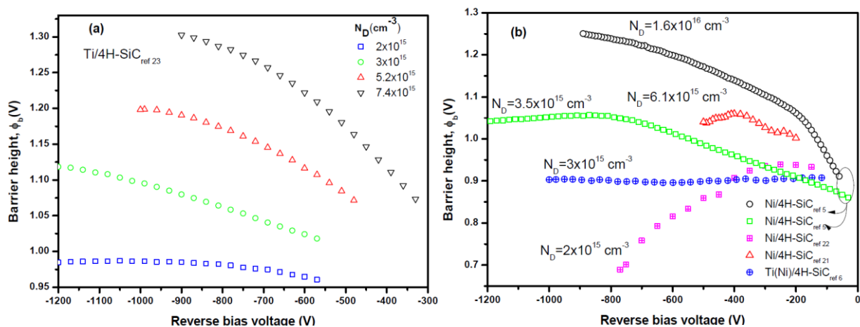
Fig. 6: Schottky Barrier Height as a Function of the Reverse Bias Voltage with Different Donor Concentrations at Room Temperature. (A) For Ti/4H-SiC ref 23 SDs, (B) For Several Metal/4H-SiC ref SDs.
