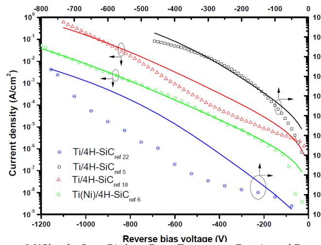
Fig. 4: Experimental and Fitted Reverse I - V Plots for Some Diodes at Room Temperature. Experimental Data are from the References as Reported in Table 1.
