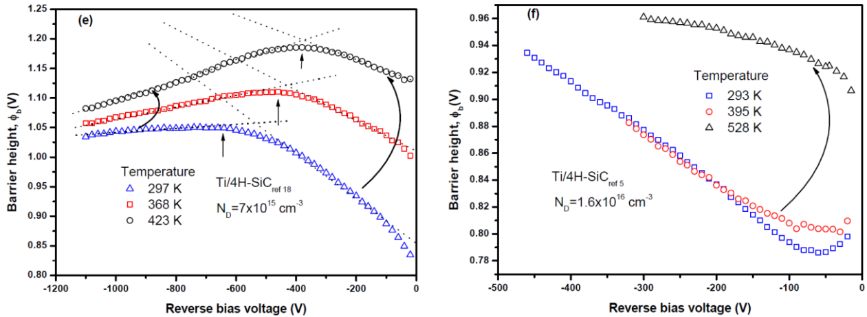
Fig. 9: Schottky Barrier Height as a Function of the Reverse Bias Voltage at Different Temperatures and Different Doping Concentration for Several Metal/4H-SiC ref SDs.
