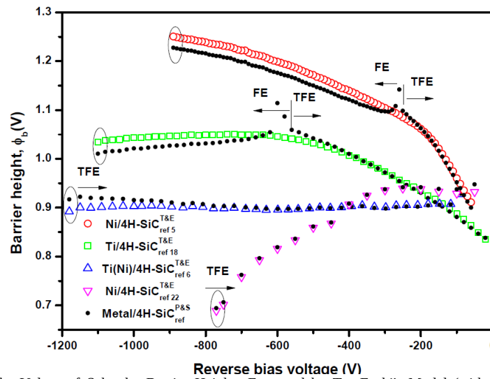
Fig. 8: Comparison between the Values of Schottky Barrier Heights Extracted by Tsu-Esaki's Model (with SBL) and the Values Extracted by Padovani-Stratton Model.
