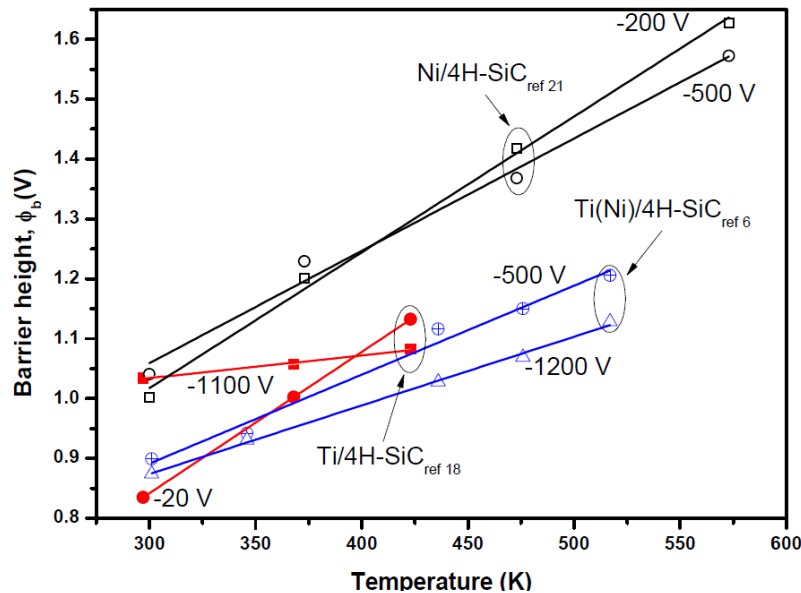
Fig. 10: The Temperature Dependence of the Barrier Height for Several Metal/4H-SiC ref Schottky Diodes at Different Reverse Bias.
