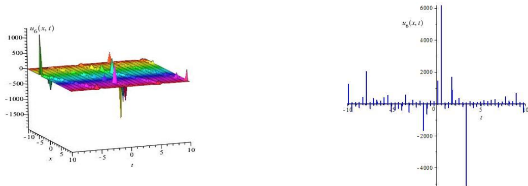
Fig. 4: Periodic Shape Solution of u_6 for \alpha=-4, \beta=-3, \delta=1, C=-1, m=2, \lambda=3, \mu=6 . the Left Figure Shows the 3D Plot and the Right Figure Shows the 2D Plot for \chi=1 .
