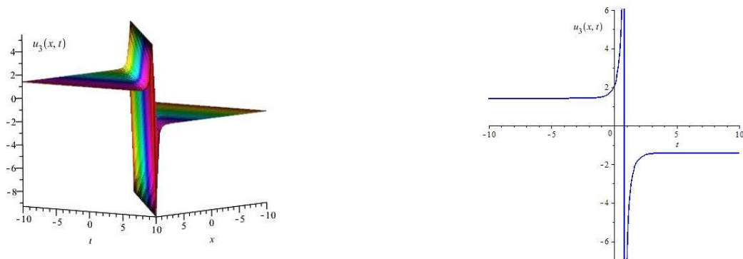
Fig. 3: Singular Kink Shape Solution of u_3 For \alpha=-2, \beta=-2, \delta=1, C=-1, m=2, \lambda=3, \mu=2 . the Left Figure Shows the 3D Plot and the Right Figure Shows the 2D Plot for \chi=1 .
