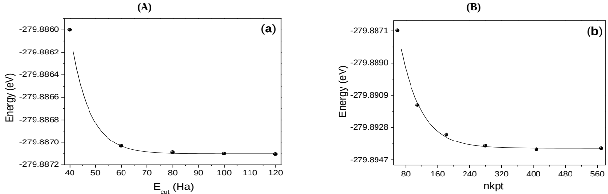
Fig. 1: Scatter Plot of Data, Plus Exponential Fitted Straight Line of E_{\text{tot}} versus Energy Cutoff and Number of K-Points of BP Compound with B1 Phase.
