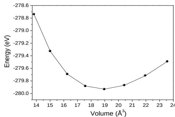
Fig. 2: Total Energy Variation with the Unit Cell Volume of Rock-Salt (B1) Phase of BP Compound.
