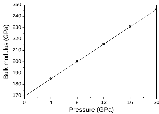
Fig. 3: Bulk Modulus Variation with the Hydrostatic Pressure of BP Compound with Rock-Salt Phase.
