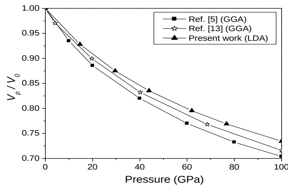
Fig. 4: Normalized Volume ( V_p/V_0 ) Versus Pressure for BP Compound with Rock-Salt Phase.
