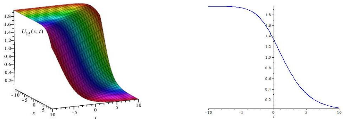
Fig. 3: Bright Kink Shape Solution of U_{15} . the Left Figure Shows the 3D Plot and the Right Figure Shows the 2D Plot For x = 1 .
