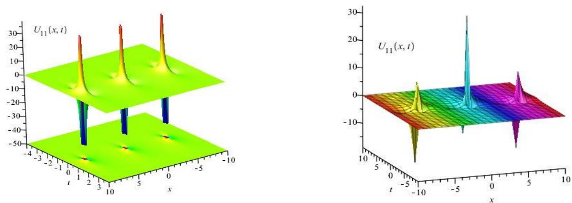
Fig. 5: Multi Rouge Wave Shape Solution of U_{11} . the Left Figure Shows the Contour Plot and the Right Figure Shows the 3D Plot.
