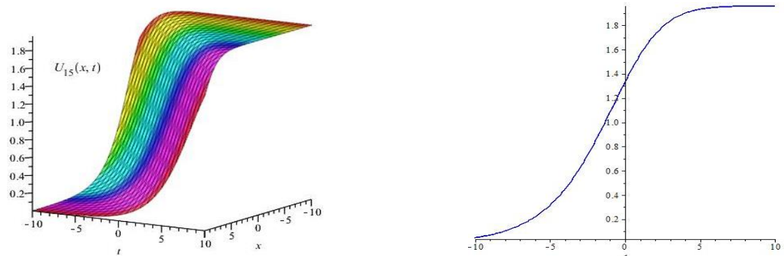
Fig. 4: Dark Kink Shape Solution of U_{15} . the Left Figure Shows the 3D Plot and the Right Figure Shows the 2D Plot For x = 1 .
