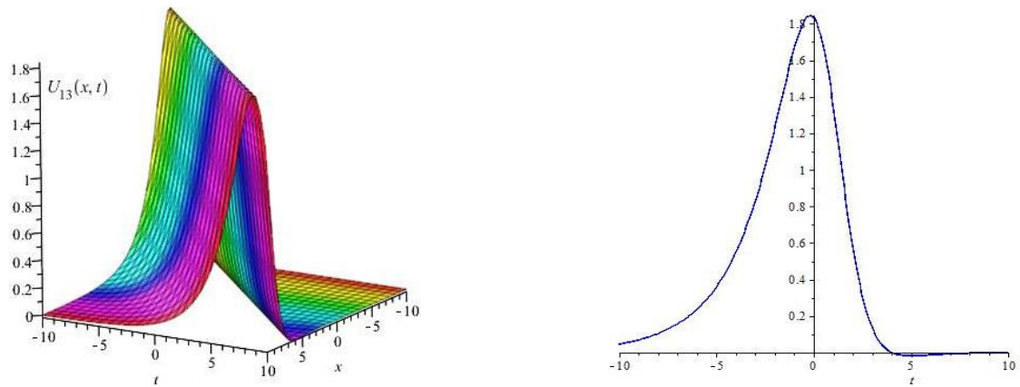
Fig. 2: Bright Bell Shape Solution of U_{13} . the Left Figure Shows the 3D Plot and the Right Figure Shows the 2D Plot For x = 1 .
