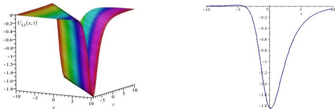
Fig. 1: Dark Bell Shape Solution of U_{13} . the Left Figure Shows the 3D Plot and the Right Figure Shows the 2D Plot For x = 1 .
