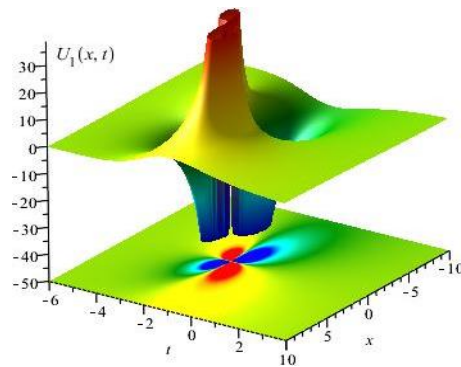
Fig. 6: Rouge Wave Shape Solution of U_1 .
