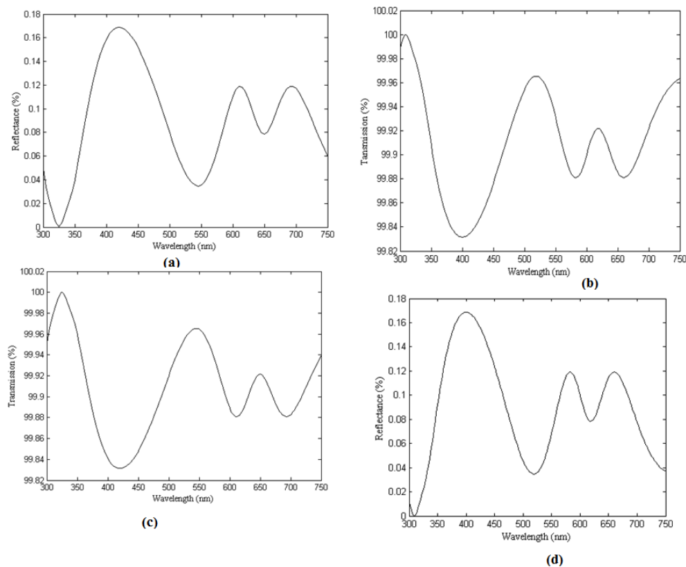
Fig. 4: Plots of Reflectance (A) and Transmittance (B) of A Double Layered Coating of Glass with \text{MgF}_2 - \text{Al}_2\text{O}_3 Designed at 650 Nm by Quarter Wavelength for Normal Incident ( \theta = 0^\circ ). These Figures Are Generated by Employing the Matrix Elements of Transformation Characteristics Matrices in The Visible Frequency Range (300nm-750nm) and Based on the Optical Thickness Obtained in Table 1. Plots of Reflectance (C) and Transmittance (D) of A Single Layered Coating of Glass with \text{MgF}_2 - \text{Al}_2\text{O}_3 Designed at 650nm by Quarter Wavelength for Normal Incident ( \theta = 60^\circ ). These Figures sre Generated by Employing the Matrix Elements of Transformation Characteristics Matrices in the Visible Frequency Range (300nm-750nm) and Based on the Optical Thickness Obtained in Table 1.
