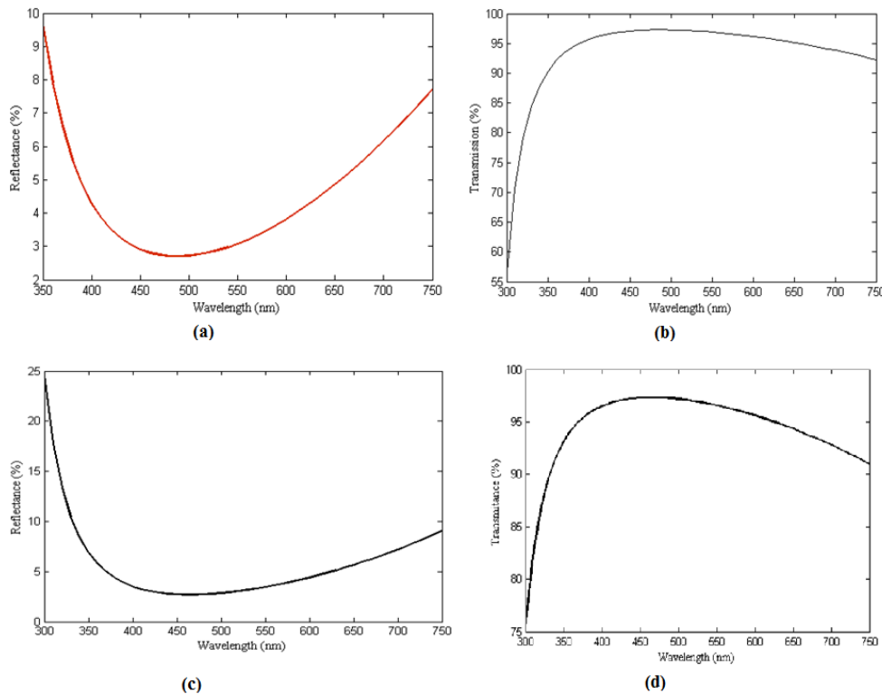
Fig. 2: Plots of Reflectance (A) and Transmittance (B) of A Single Layered Coating of Glass with \text{MgF}_2 Designed at 650nm by Quarter Wavelength for Normal Incident ( \theta = 0^\circ ). These Figures are Generated by Employing the Matrix Elements of Transformation Characteristics Matrices in the Visible Frequency Range (300nm-750nm) and Based on the Optical Thickness Obtained in Table 1. Plots of Reflectance (C) and Transmittance (D) of A Single Layered Coating of Glass with \text{MgF}_2 Designed at 650nm by Quarter Wavelength for Normal Incident ( \theta = 60^\circ ). These Figures are Generated by Employing the Matrix Elements of Transformation Characteristics Matrices in the Visible Frequency Range (300nm-750nm) and Based on the Optical Thickness Obtained in Table 1.
