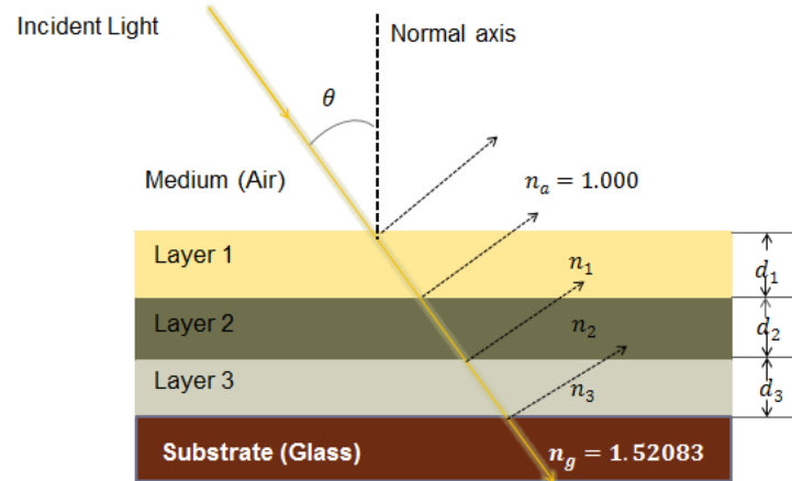
Fig. 1: The Schematic Diagram of the System Design in Triple Anti-Coating Representation with the Layer Thickness D_1 , D_2 and D_3 . the Corresponding Value for These Optical Thicknesses Will Be Determined for A Matching Materials Based on the Quarter-Quarter-Quarter (-Q-Q-Q) Wavelength Theory
