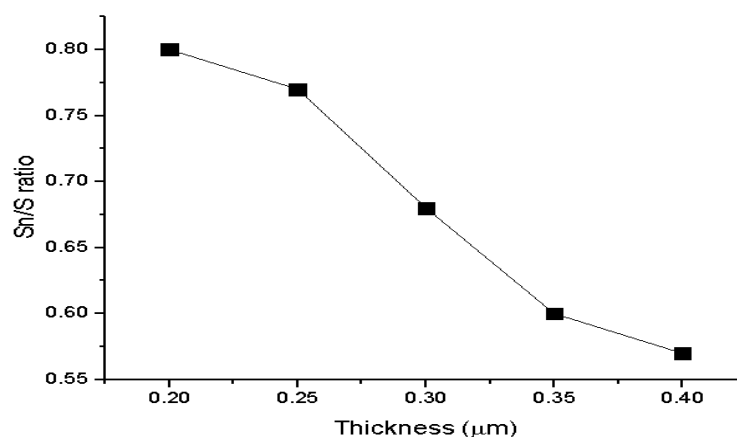
Fig. 3: Sn/S Atomic Percent (at. %) Ratio as a Function of Film Thickness.
