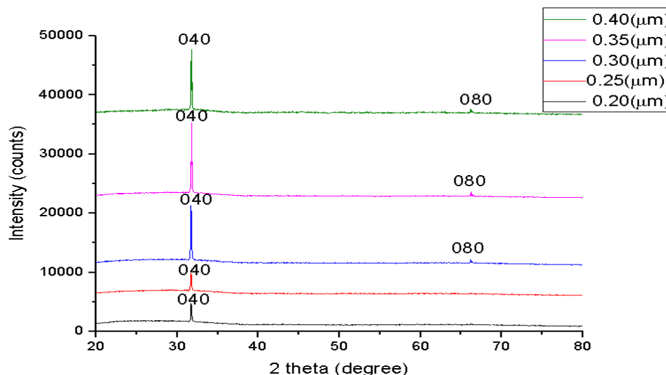
Fig. 4: XRD Pattern for SnS Thin Films of 0.20 \mu\text{m} , 0.25 \mu\text{m} , 0.30 \mu\text{m} , 0.35 \mu\text{m} and 0.40 \mu\text{m} Thickness.
