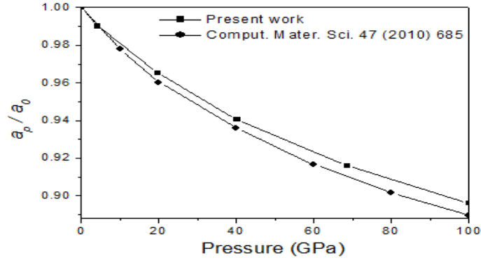
Fig. 1: Normalized Lattice Parameter ( a_p/a_0 ) Versus Pressure.
