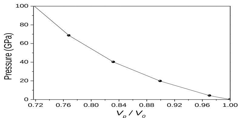
Fig. 3: Pressure versus ( V_p/V_0 ) of BP with B1 Phase.
