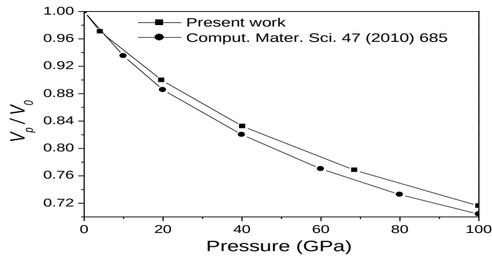
Fig. 2: Normalized Volume ( V_p/V_0 ) Versus Pressure.
