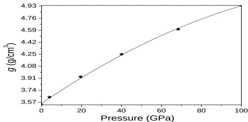
Fig. 4: Crystal density Versus Pressure of BP Up to 100 GPa.
