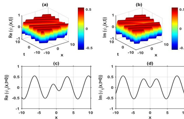
Fig. 1: A)-B) 3D Illustrations of the Eq. (10) for the Choosing Arbitrary Parameters C = 1, A = 3, K = -1, D = 1, \Sigma = 1 Within -10 \leq X \leq 10, -10 \leq T \leq 10 , and (C)-(D) 2D Line Illustrations of (A)-(B) at T = 0 , Respectively.
