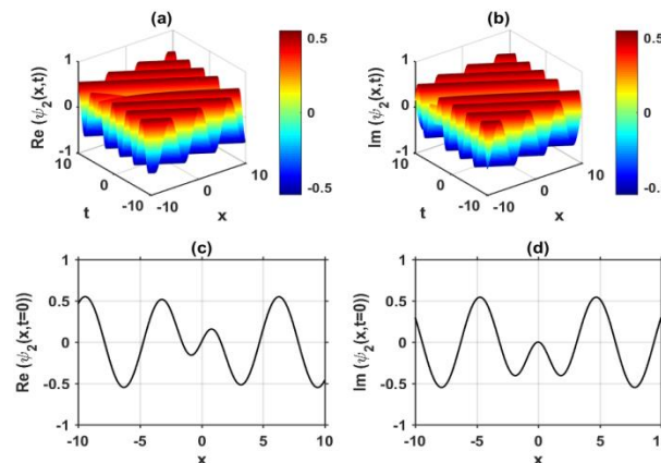
Fig. 2: A)-B) 3D Illustrations of the Eq. (11) for the Choosing Arbitrary Parameters C = 1, A = 3, K = -1, D = 1, \Sigma = 1 Within -10 \leq X \leq 10, -10 \leq T \leq 10 , and (C)-(D) 2D Line Illustrations of (A)-(B) at T = 0 , Respectively.
