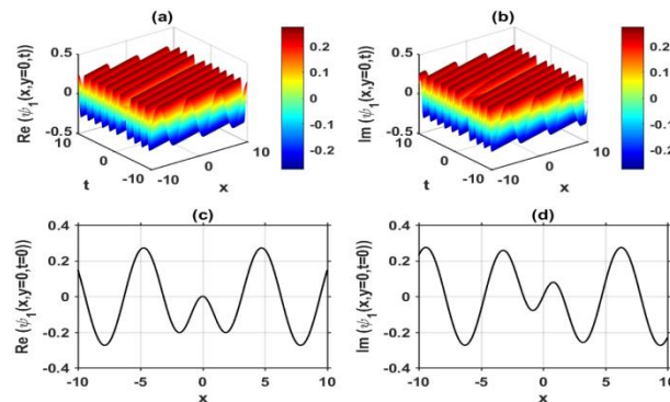
Fig. 3: A)-B) 3D Illustrations of the Eq. (15) for the Choosing Arbitrary Parameters p = 1, b_1 = 1, q = 1, b_2 = 1, \alpha = 1, \beta = 1, A = 3, d = 1, a = 1, y = 0 within -10 \leq x \leq 10, -10 \leq t \leq 10 , and C)-D) 2D Line Illustrations of A)-B) at y = 0, t = 0 , Respectively.
