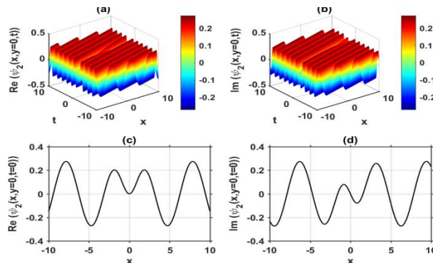
Fig.4: A)-B) 3D Illustrations of the Eq. (16) for the Choosing Arbitrary Parameters p = 1, b_1 = 1, q = 1, b_2 = 1, \alpha = 1, \beta = 1, A = 3, d = 1, a = 1, y = 0 within -10 \leq x \leq 10, -10 \leq t \leq 10 , and C)-D) 2D Line Illustrations of A)-B) at y = 0, t = 0 , Respectively.
