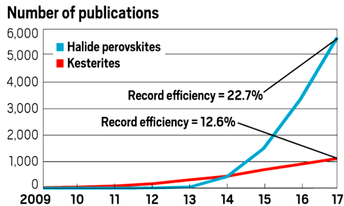
Fig. 1: The Record Efficiency of Perovskite Solar Cells in the Laboratory [4].
