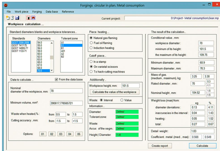
Fig. 6: The Study of Metal Process GOSH Forging Parts Gear and Calculate the Utilization Rate of Metal.
