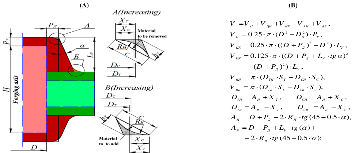
Fig. 2: Modeling Assignment Allowances and Overlaps the Outer Sides of the Elements of Forging (A) and the Expressions for Calculating Their Volumes (B).
