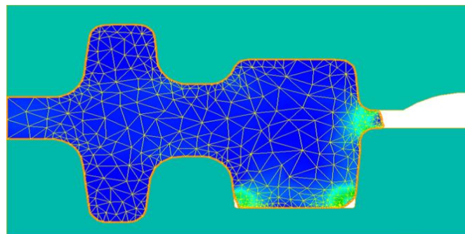
Fig. 5: The Process of Forming of the Forging at the Final Forging the Transition.
