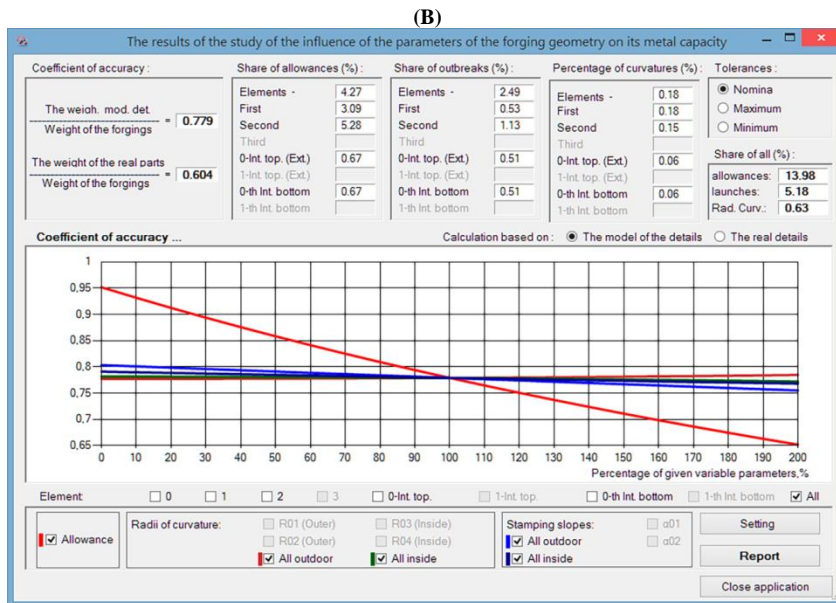
Fig. 4: A Study of the Influence of the Values of Allowances, Tolerances, Overlaps on the Value of the Coefficient of Precision Forgings In General (A) and Separately for Each of the Forms (B) Forming A Forging.
