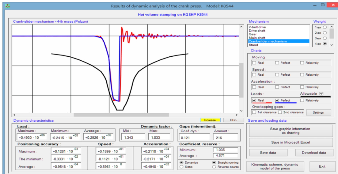
Fig. 7: Modeling of Dynamic Processes in KGSP.
