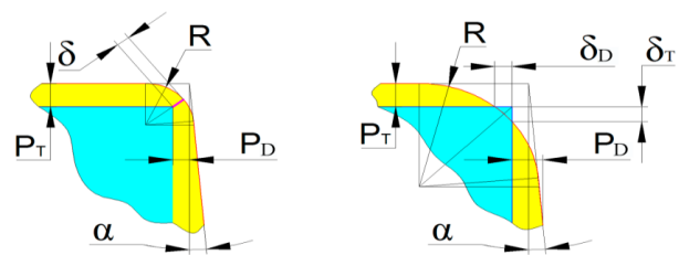
Fig. 1: To Calculate the Values of Allowances.
