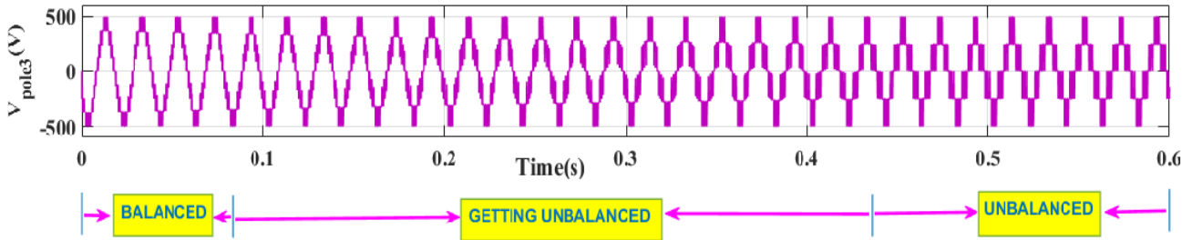
Fig. 2: Transition of DCMLI level from five to three
