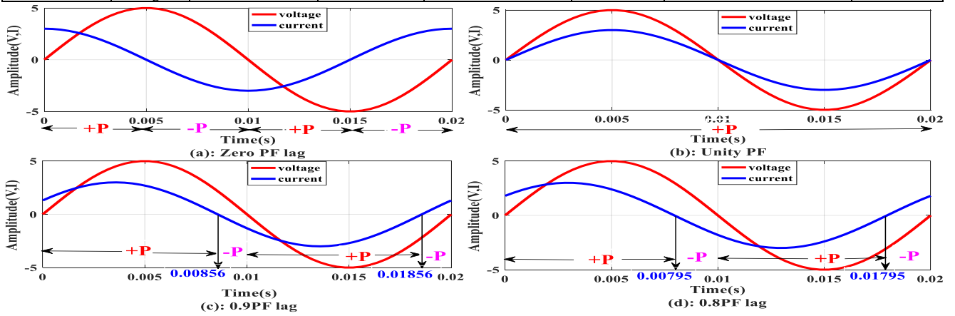
Fig.5: load current and voltages of 5level DCMLI for a) ZPF b) UPF c) 0.9PF lag d) 0.8PF lag
