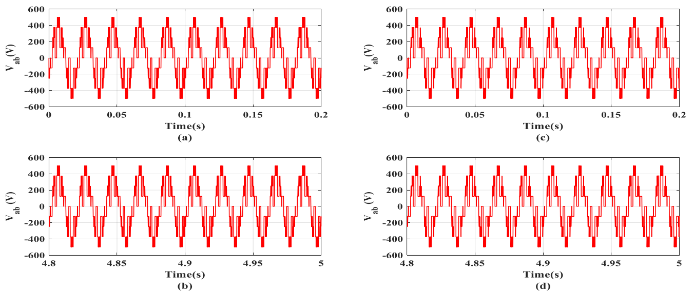
Fig. 11: Line Voltages of Hybrid PWM technique with M_a=1.0 for 0.8PF lag load, p_w=5.7\% (a) Initial cycles (b) final cycles For 0.9PF lag load p_w=6.7\% (c) initial cycles (d) final cycles
