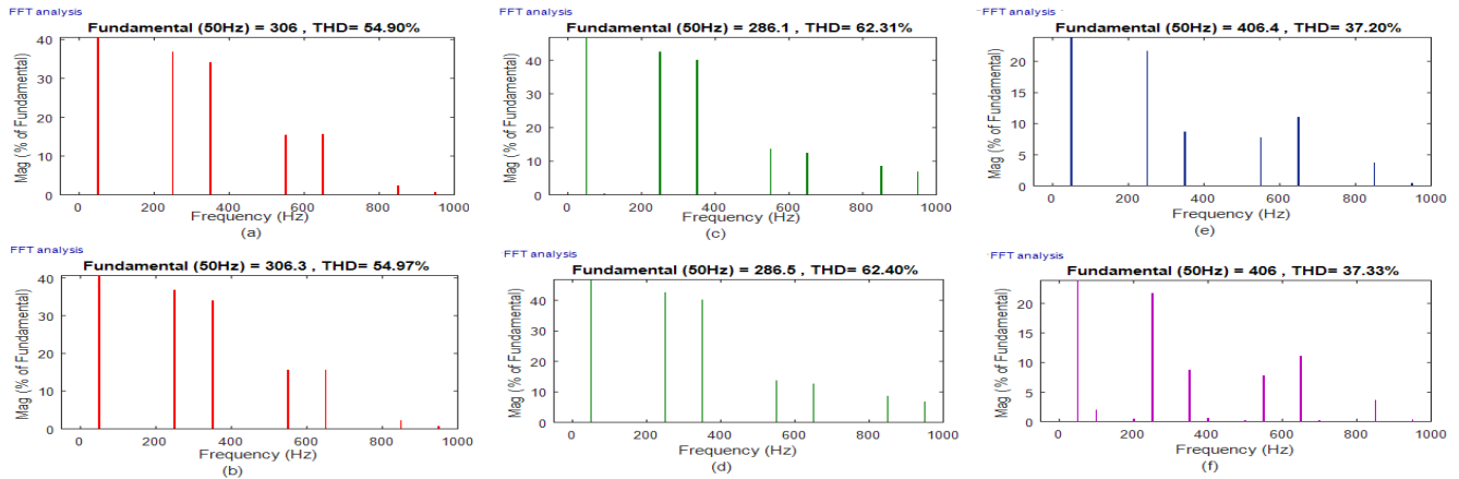
Fig. 12: THD for PF=0.8lag (a) initial cycles of Hybrid PWM (b) final cycles of Hybrid PWM (e) final cycles of SPWM for PF=0.9lag (c) initial cycles of Hybrid PWM (d) final cycles of Hybrid PWM (f) final cycles of SPWM
