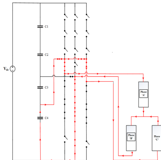
Fig. 7: 101 switching state of 5-level DCMLI
