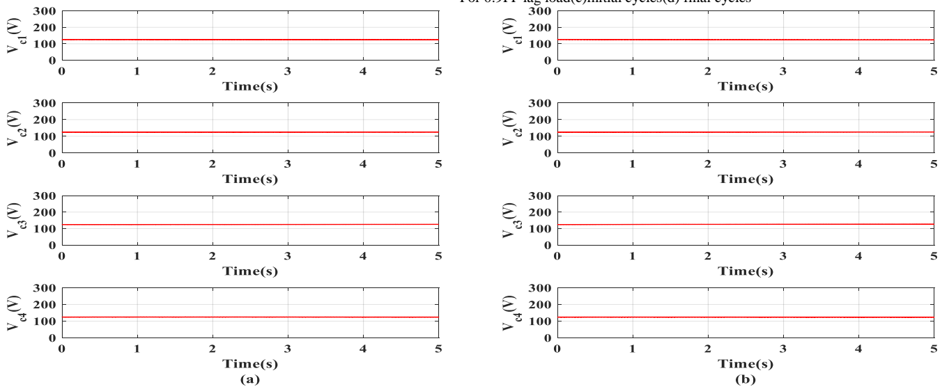
Fig. 10: Capacitor Voltages of Hybrid PWM technique for (a) 0.8PF lag load with M_a=1.0 , p_w=5.7\% (b) for 0.9PF lag load with M_a=1.0 , p_w=6.7\%
