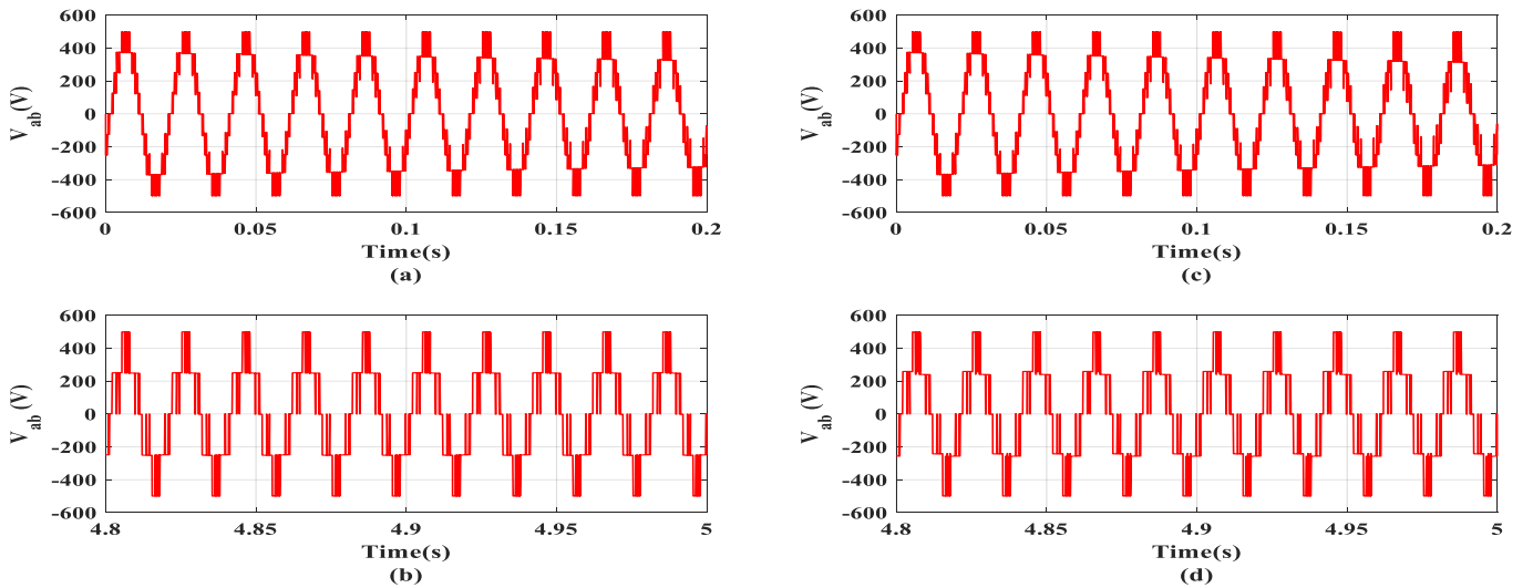
Fig. 9: Line Voltages of CBPWM technique with M_a=1.0 for 0.8PF lag load (a) Initial cycles (b) final cycles For 0.9PF lag load (c) initial cycles (d) final cycles
