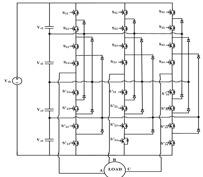
Fig. 1: Schematic of five-level DCMLI
