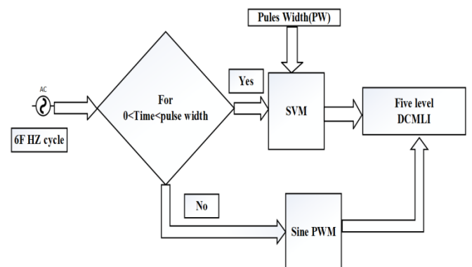
Fig. 4: Block diagram of Hybrid PWM technique
