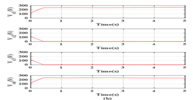
Fig. 8: Capacitor voltages of CBPWM technique (a) for 0.8PF lag load with Ma=1.0 (b) for 0.9PF lag load with Ma=1.0
