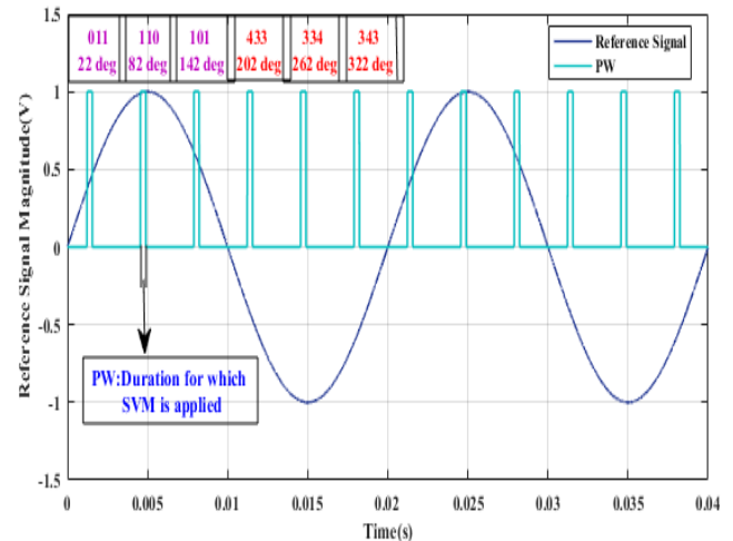
Fig. 3: Hybrid PWM technique
