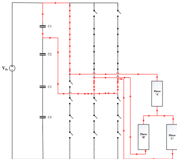
Fig. 6: 433 switching state of 5-level DCMLI
