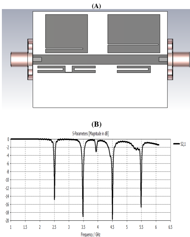
Fig. 1: (A) Layout of the Tag for Encoding ID “10101010”, (B) Simulated Insertion Loss ( S_{21} ) for the Tag with ID 10101010.
