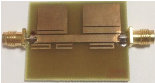
Fig. 7: Hardware Implementation of the Tag for Encoding the ID "10101010".
