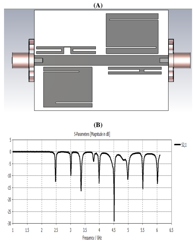
Fig. 5: (A) Layout of the Tag For Encoding the ID “11111111”, (B) Simulated Insertion Loss ( S_{21} ) for the Tag with ID 11111111.
