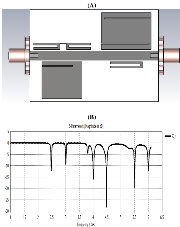
Fig. 3: (A) Layout of the Tag for Encoding ID “11011011”, (B) Simulated Insertion Loss ( S_{21} ) for the Tag with ID 11011011.
