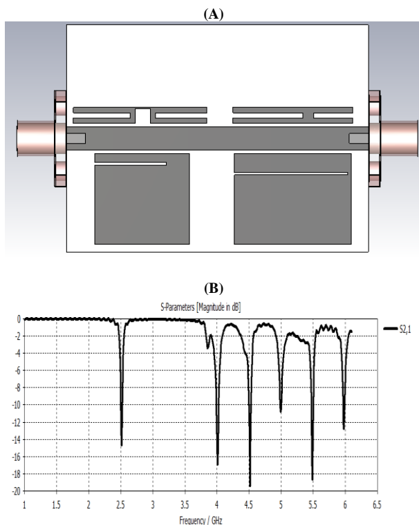
Fig. 4: (A) Layout of the Tag for Encoding ID “10011111”, (B) Simulated Insertion Loss ( S_{21} ) for the Tag with ID 10011111.
