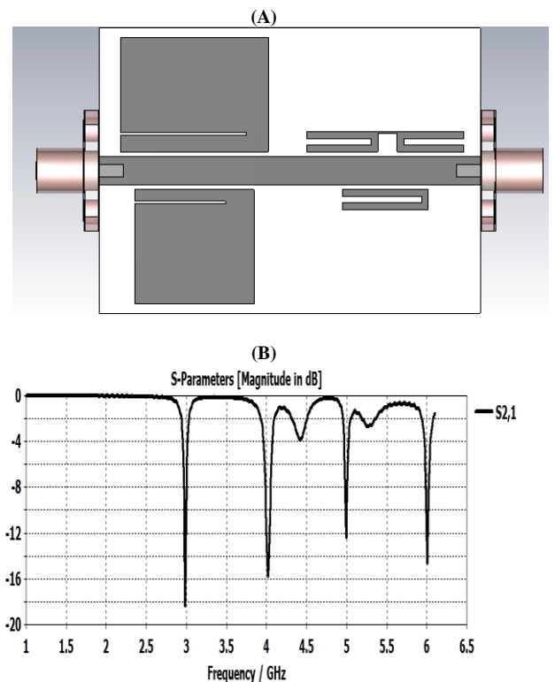
Fig. 2: (A) Layout of the Tag for Encoding ID “01010101”, (B) Simulated Insertion Loss ( S_{21} ) for the Tag with ID 01010101.
