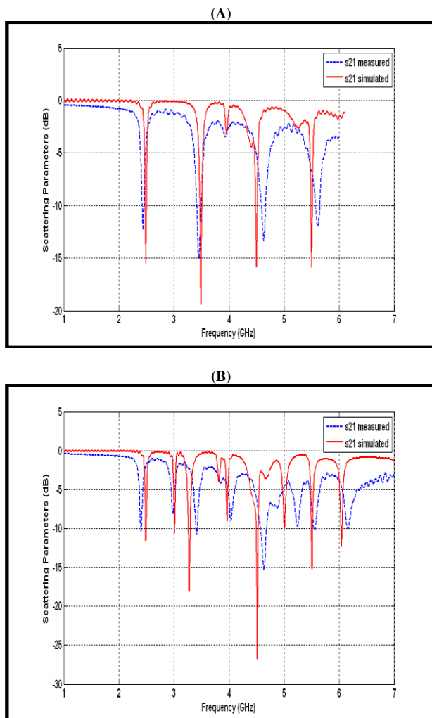
Fig. 8: Comparison of Simulated and Measured S_{21} . (A) Encoding the ID "10101010", (B) Encoding the ID "11111111".
