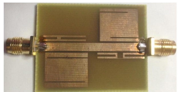
Fig. 6: Hardware Implementation of the Tag for Encoding the ID “11111111”.
