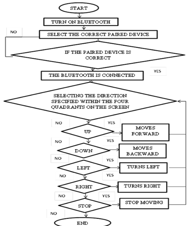
Fig. 7: Flow-Chart for Touch Mode.
