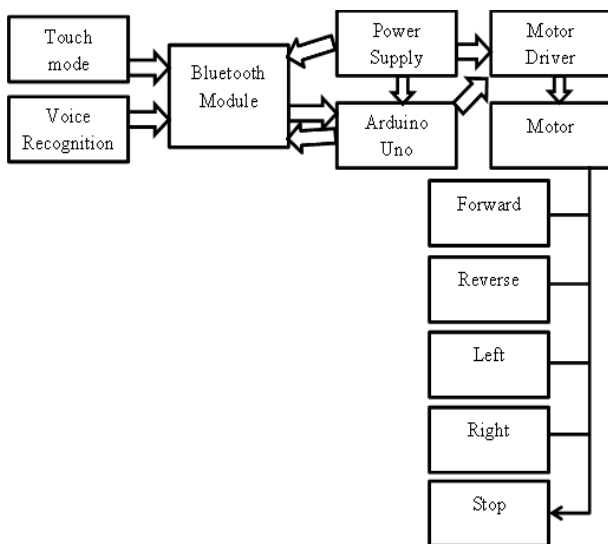
Fig. 5: Smart Wheelchair Work-Flow Process.
