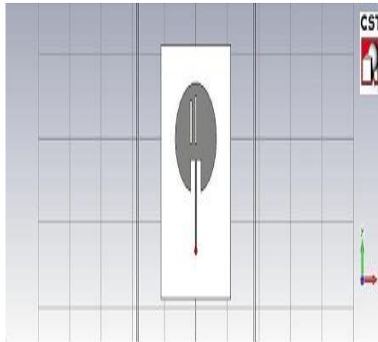
Fig.5 CMPA With 2slit-slot for Multiband Application
