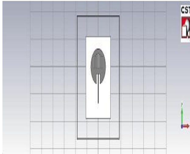
Fig.9. CMPA With 6 Slit-slot for Multiband Application
