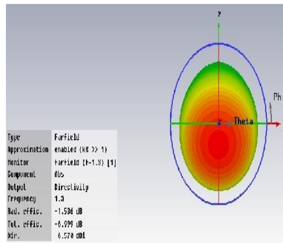
Fig. 3 Radiation pattern of simple circular patch at 1.3GHz
