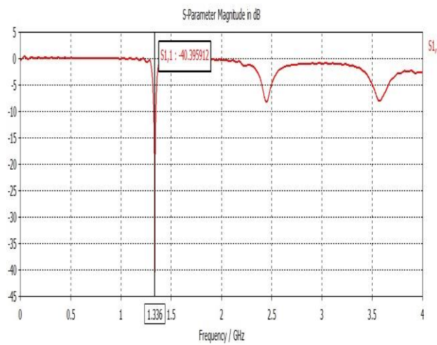
Fig. 2 Return losses vs. frequency for circular patch without slot
