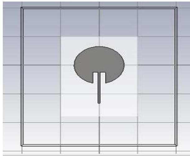
Fig. 1 Circular microstrip patch
