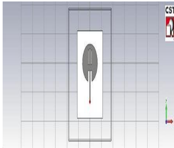
Fig.7. CMPA With 3Slit-slot for Multiband Application
