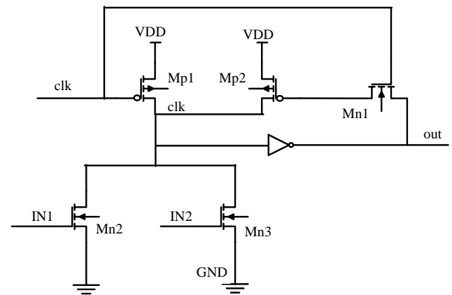
Fig. 2: The suggested domino-logic based circuit. The Mp3 transistor and two inverter gates were eliminated.
