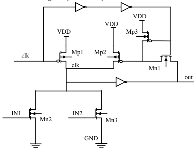
Fig. 1: The original high speed domino-logic based circuit
