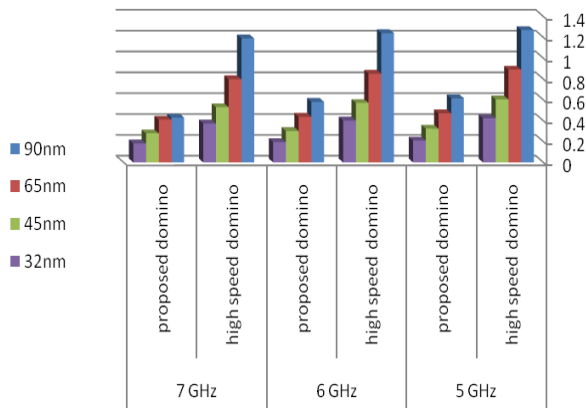
Fig. 4: PDP comparison between high speed domino logic and proposed domino logic in different technologies when the keeper transistor channel length is triple the minimum size.
