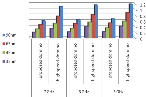
Fig. 3: PDP comparison between high speed domino logic and proposed domino logic in different technologies when the keeper transistor channel length is minimum size.
