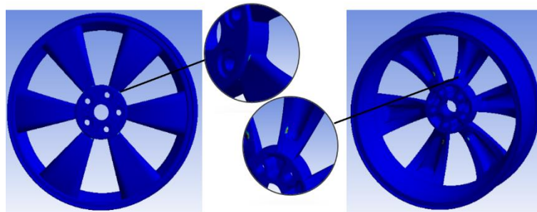
Fig. 5: The Minimum Fatigue Life Area.
