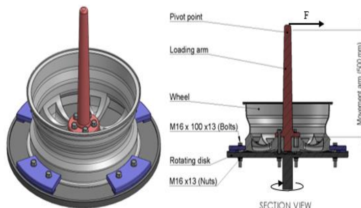
Fig. 2: Assembly Drawing for Dynamic Cornering Fatigue Test Based on ISO-3006.
