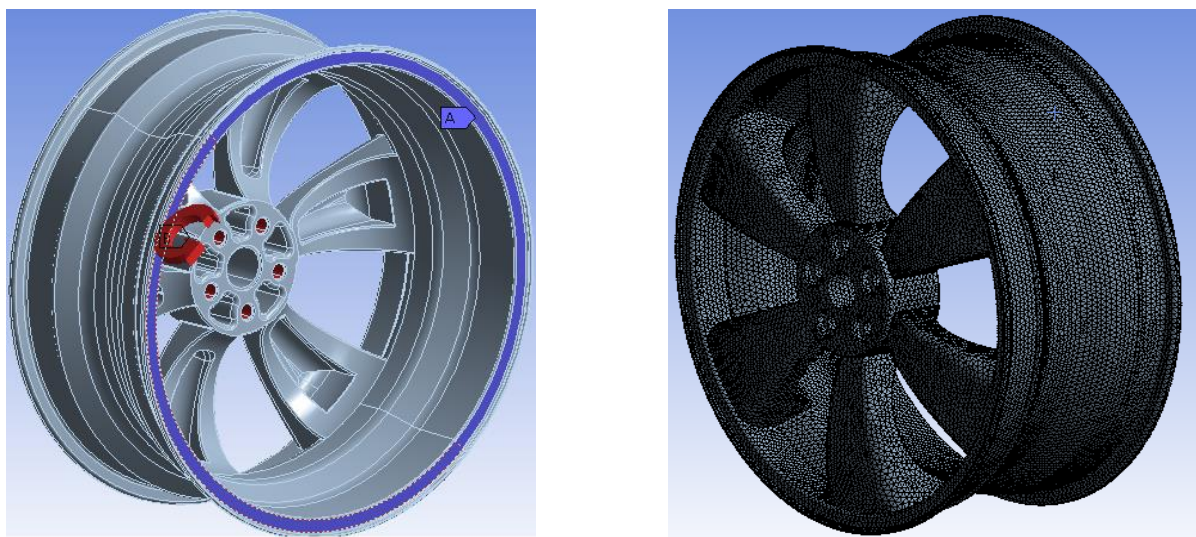
Fig. 3: The Model: A) Initial Loading B) Mesh.
