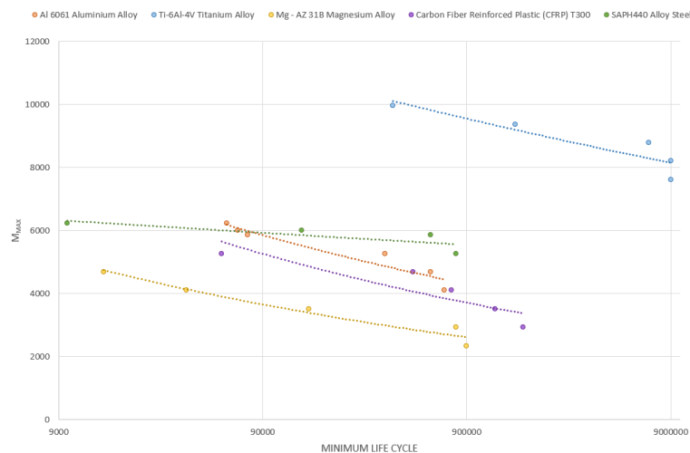
Fig. 6: The Minimum Life Cycle for Each Moment.
