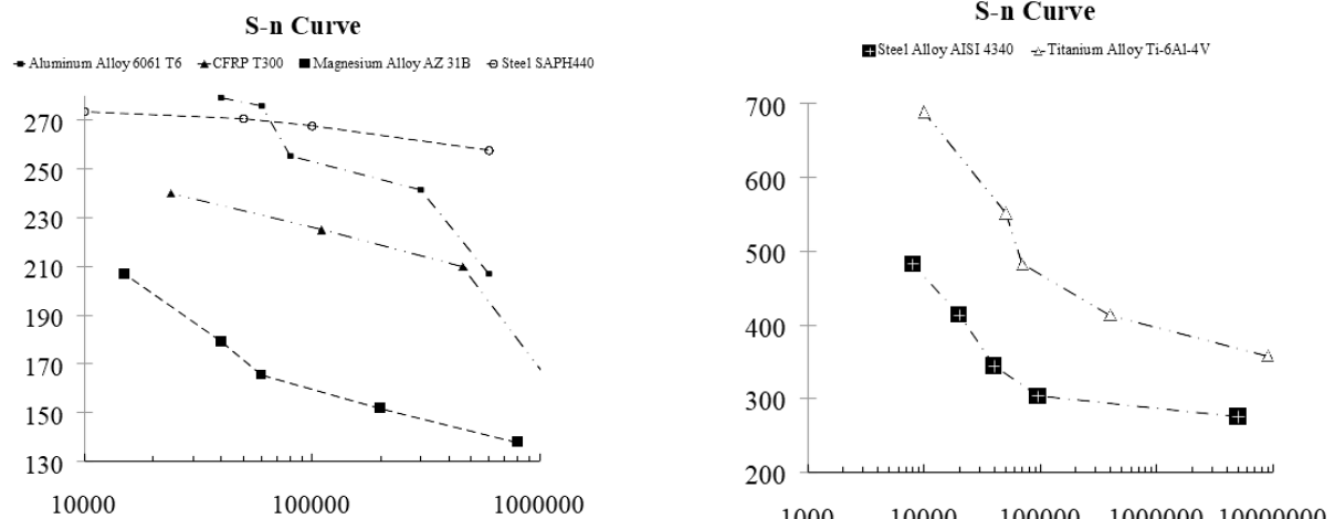
Fig. 1: S-N Curve of Selected Materials.
