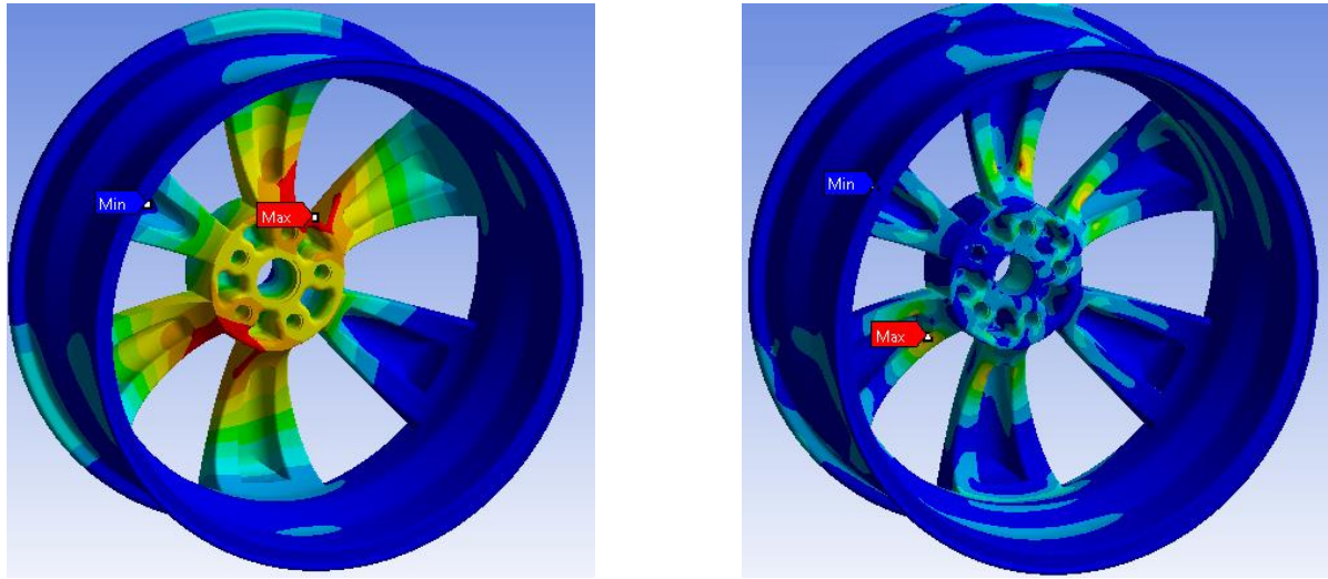
Fig. 4: Static Results: A) Deformation B) Von-Mises Stress.
