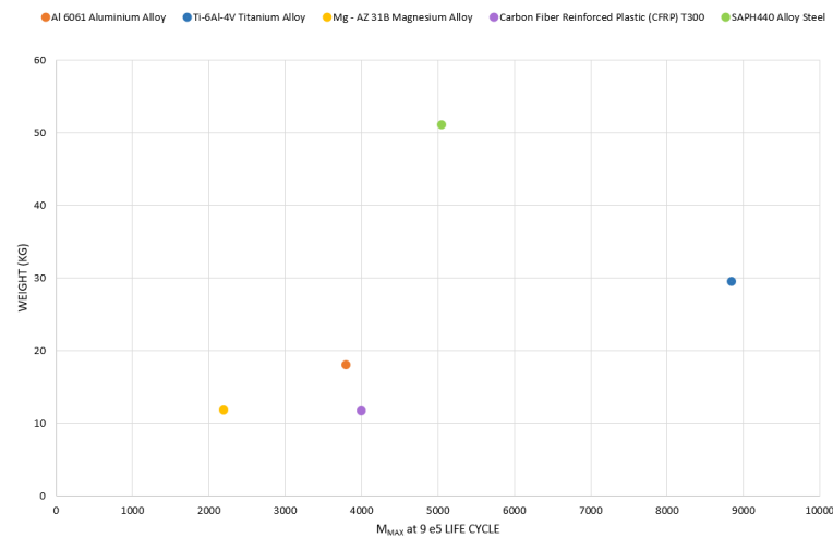
Fig. 7: The Maximum Moment at 9 * 10^5 Life Cycle Versus Weight.
