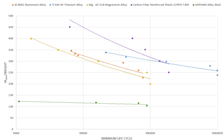
Fig. 8: The Minimum Life Cycle Versus Moment/Weight.
