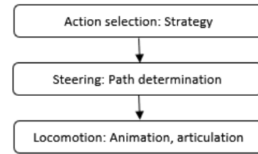
Fig. 1: Behavior Hierarchy
