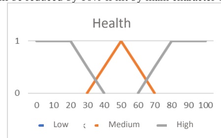
Fig. 3: Health variable
