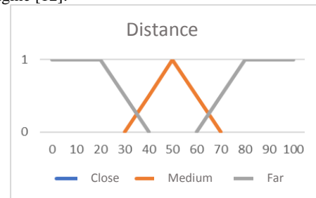
Fig. 2: Distance variable
