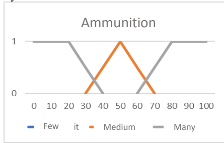
Fig. 4: Ammunition variable
