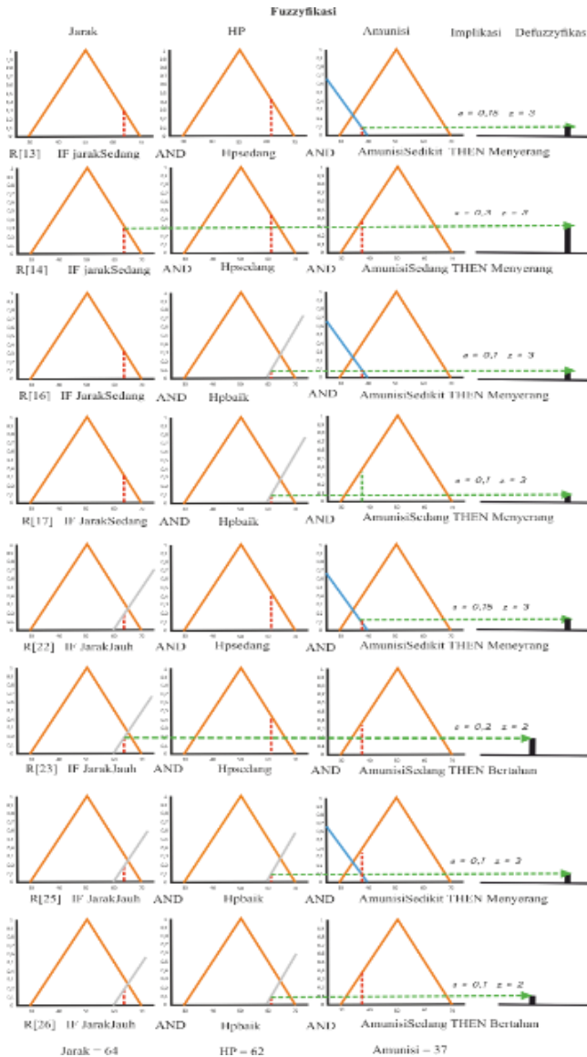
Fig. 6: Sugeno Fuzzy Calculation Curve
