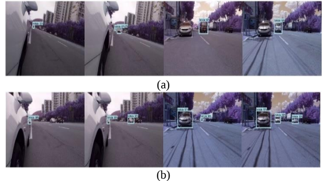
Fig. 5. The frame sequence result of the Faster R-CNN, (a) the result of true positive, (b) the result of false positive.
