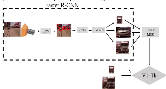
Fig. 1. The architecture of proposed algorithm.
