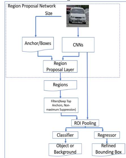
Figure 2. The Architecture of Faster R-CNN
