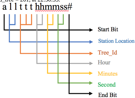
Fig. 5: Log Data Structure for Tracking System
