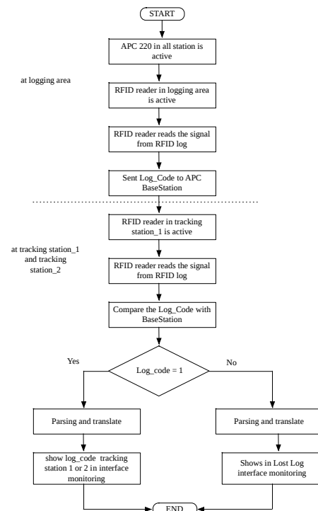
Fig.8: Flowchart of The Proposed System
