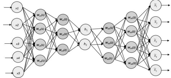
Fig 5. Deep SDAE architecture
