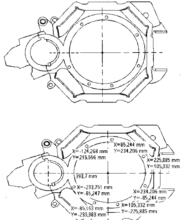
Fig. 2: Axle cap of GE 761 traction motor
