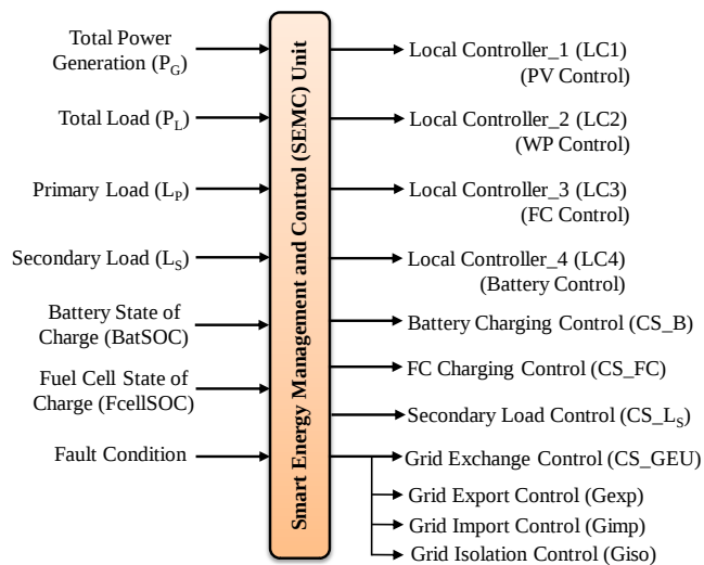
Fig. 5: Typical inputs and outputs to design SEMC strategy
