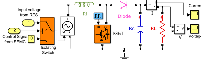
Fig. 3: Local controller (LC) model developed in MATLAB/Simulink.
