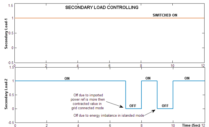
Fig. 11: Secondary load control based on SEMC commands
