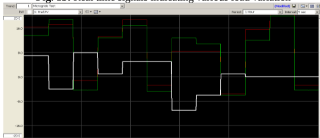
Fig. 14: Power exchange between microgrid and utility grid
