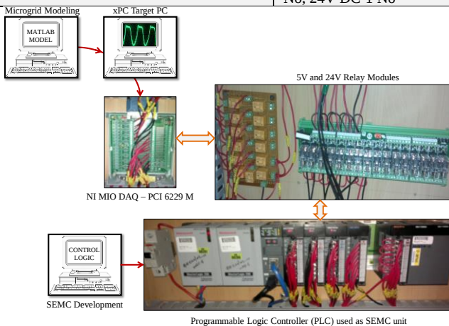
Fig. 7: Proposed HIL setup for real-time implementation of SEMC
