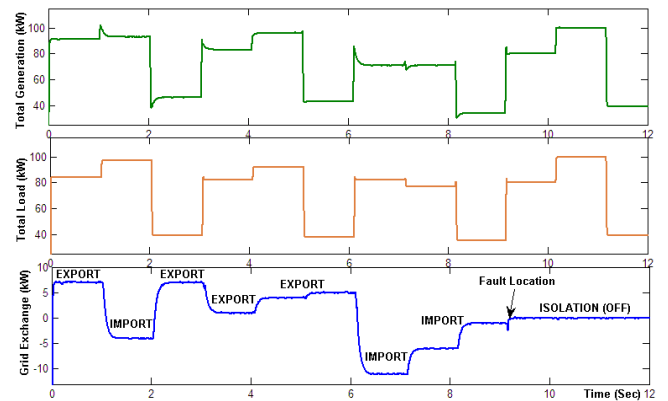
Fig. 10: Grid exchange based on SEMC commands
