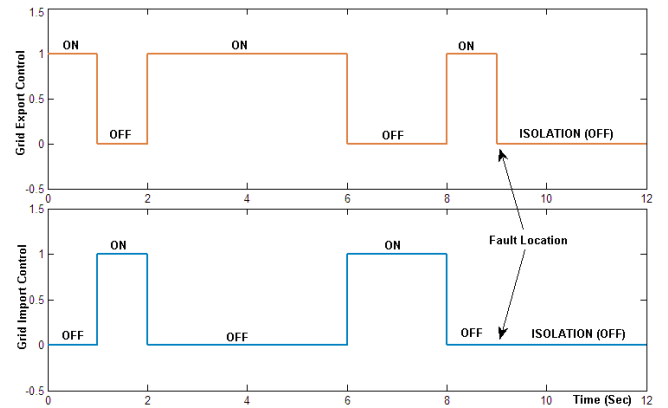
Fig. 9: SEMC unit control signals to grid exchange unit
