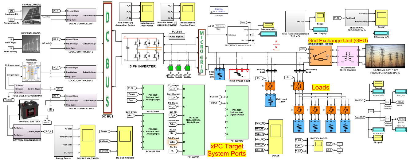
Fig. 2: Microgrid architecture modeled in MATLAB/Simulink for HIL testing.
