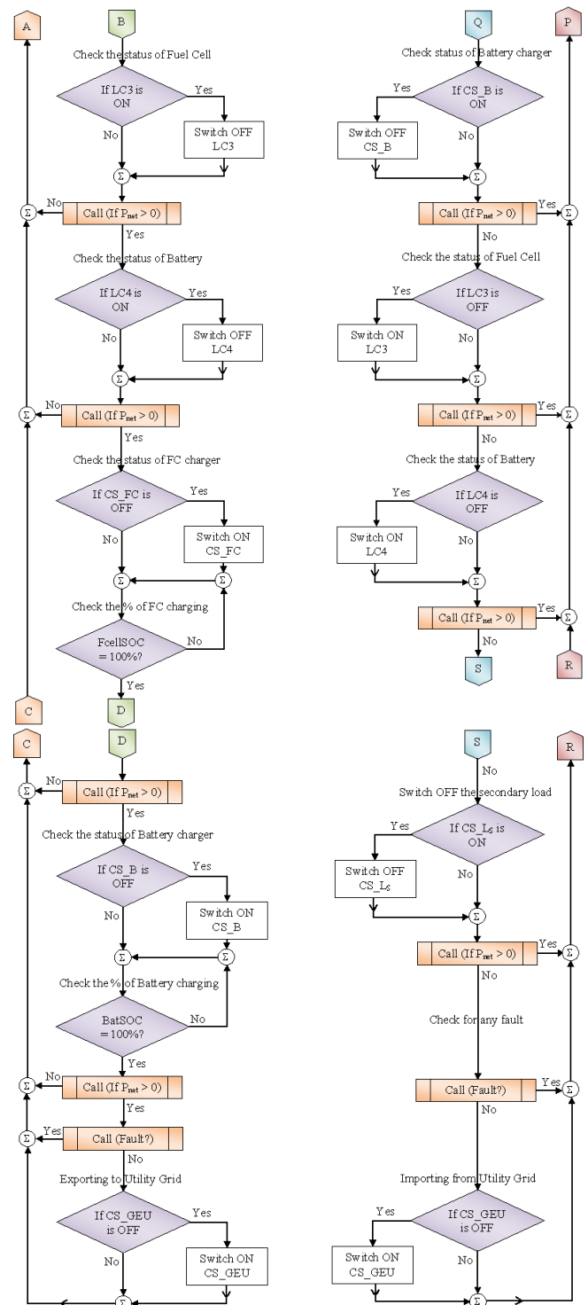
Fig. 6: Proposed algorithm for SEMC design
