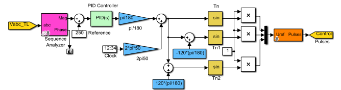
Fig. 4: Closed loop PID control loop to produce inverter firing pulses
