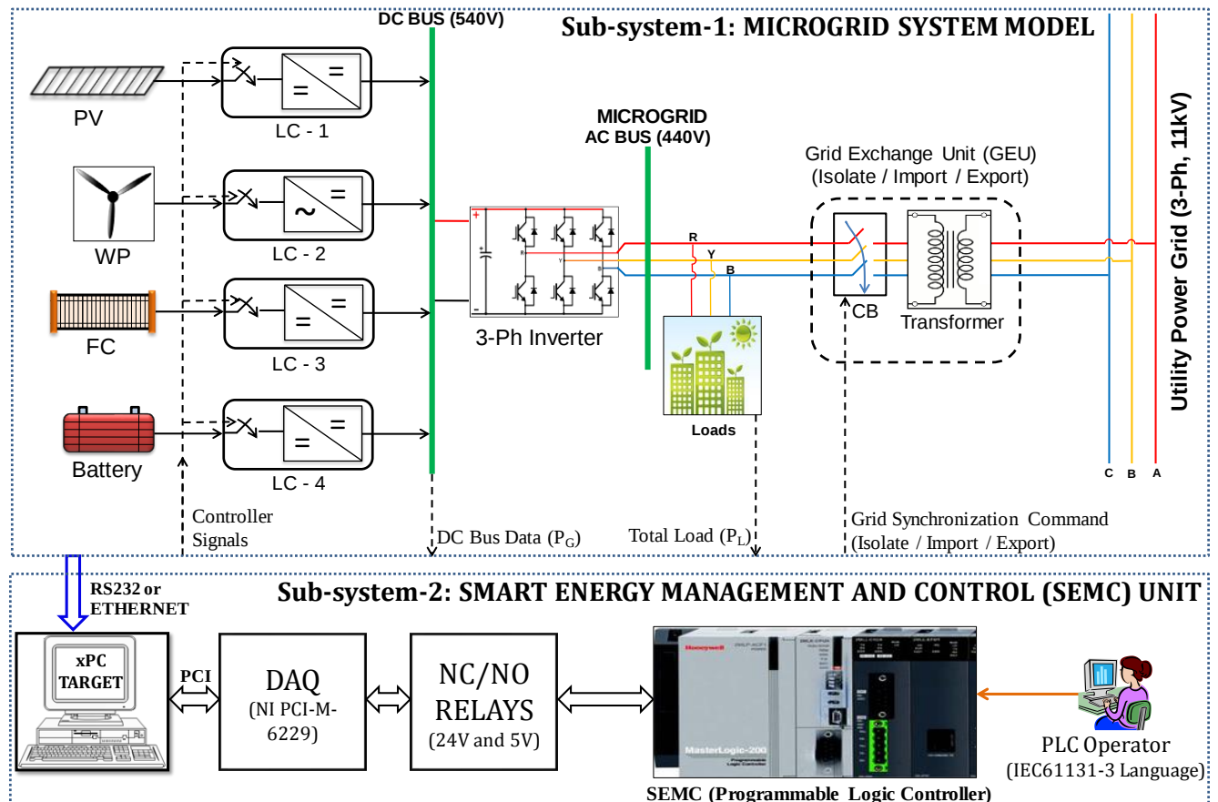
Fig. 1: Proposed hardware in the loop (HIL) test setup for real-time energy management and control of microgrids.
