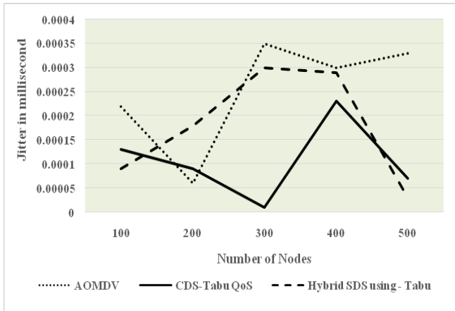
Figure 5: Jitter
