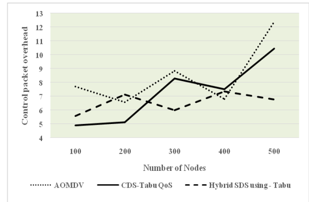
Figure 6: Control Packet Overhead
