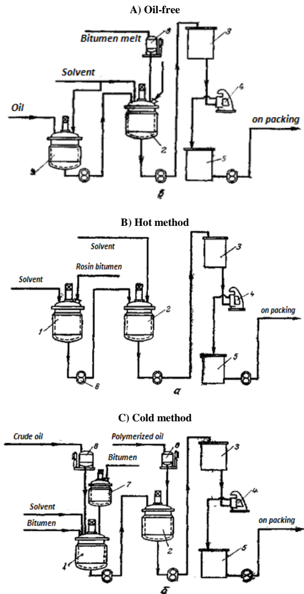
Fig. 2: The Scheme of Production of Bituminous Varnishes: 1 - Reactor; 2 - Mixer; 3 - Pressure Tank; 4 - Super-Centrifuge; 5 - Receiving Tank; 6 - Pump; 7 - Melter; 8 Gauges on Scales; 9 - Polymerizer.
