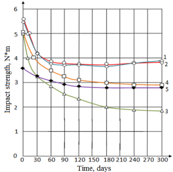
Fig. 6: Change in Impact Strength of Bituminous Coatings in Water at 50°C.
