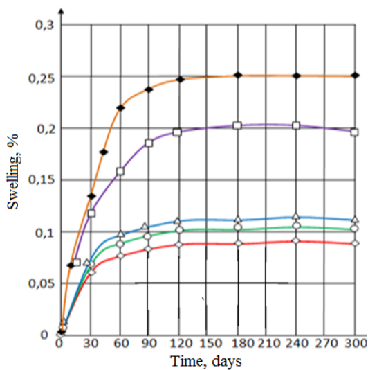
Fig. 4: Swelling of Bitumen Coatings in Water at 50°C.
