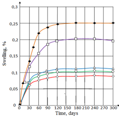
Fig. 3: Swelling of Bituminous Coatings in Water at 25°C.
