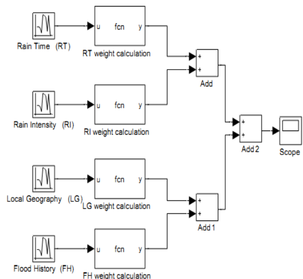
Fig. 2: MATLAB Simulink model of proposed FFWS algorithm
